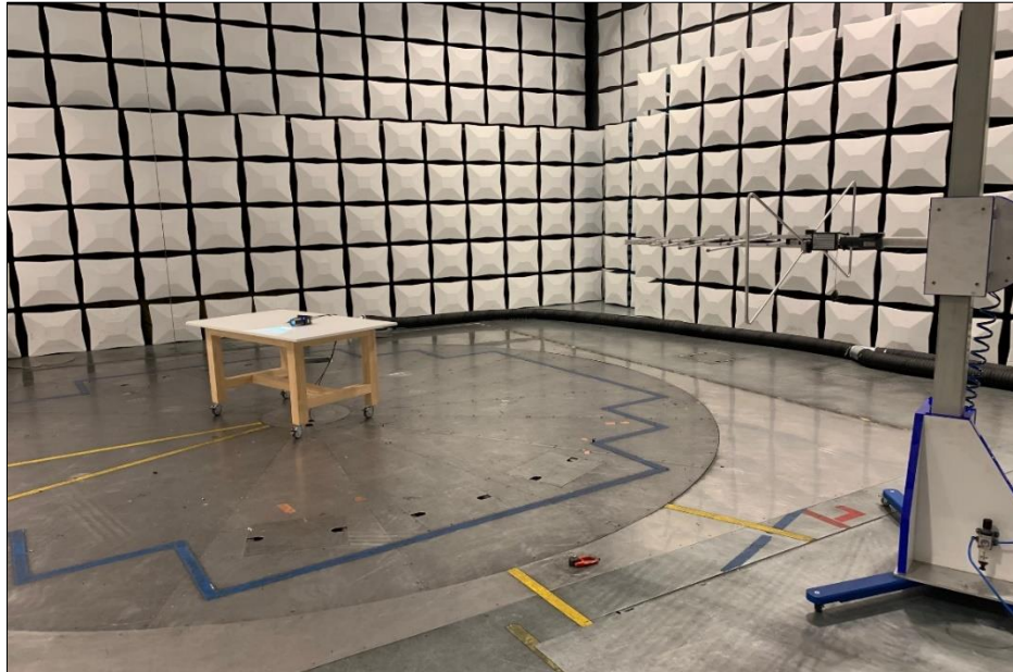
Radiated emissions
