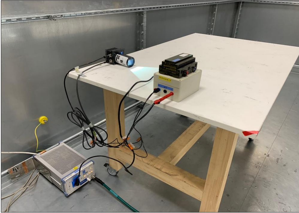
Conducted emissions on AC line
