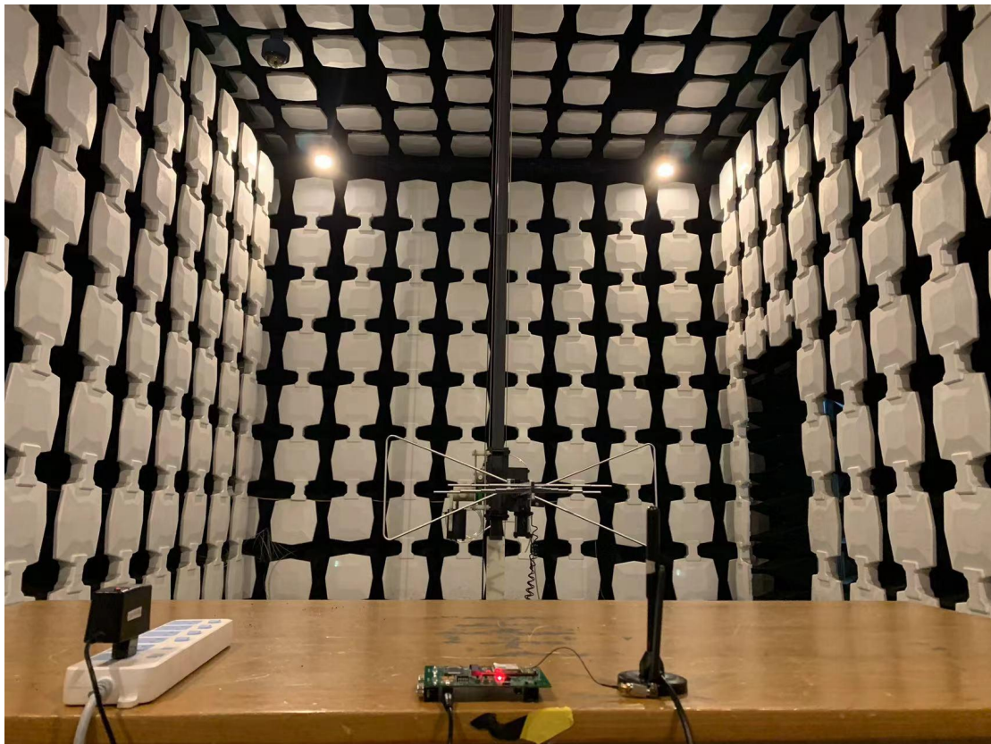
A7672SA miniPCIE RE 30MHz-1GHz
