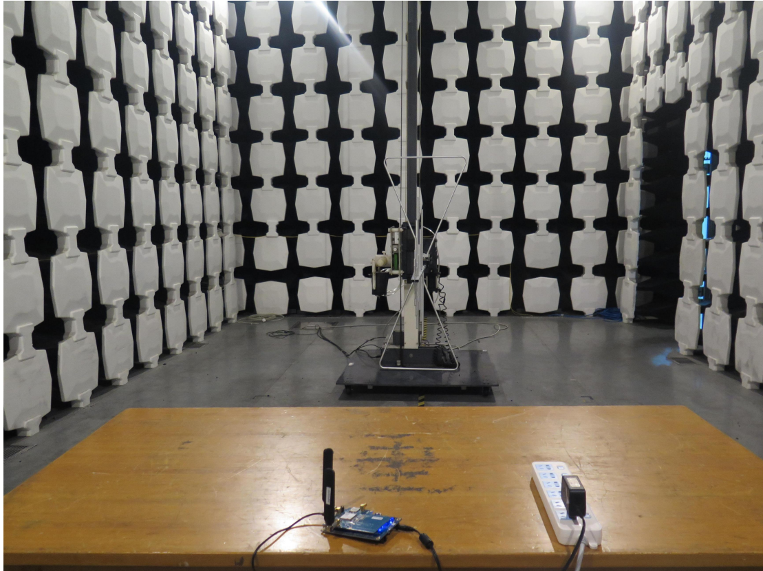
A7672SA RE 30MHz-1GHz
