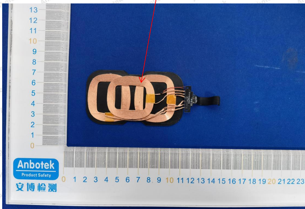
Tx Coil
