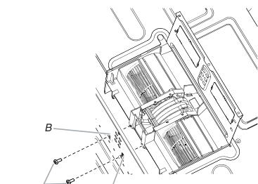
A. Screws B. Blower motor screw holes
