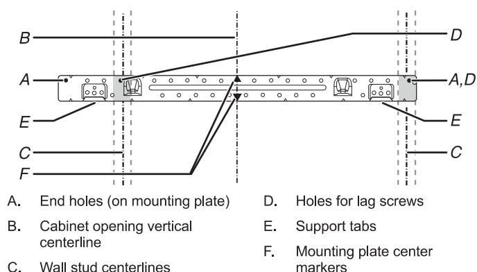
Wall Stud at End Holes Figure 4
