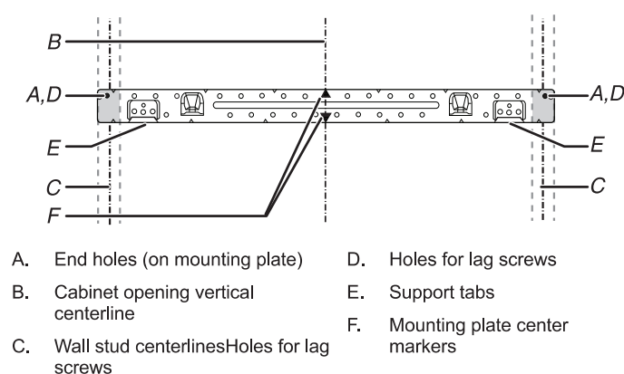
Wall Stud at End Holes Figure 4
