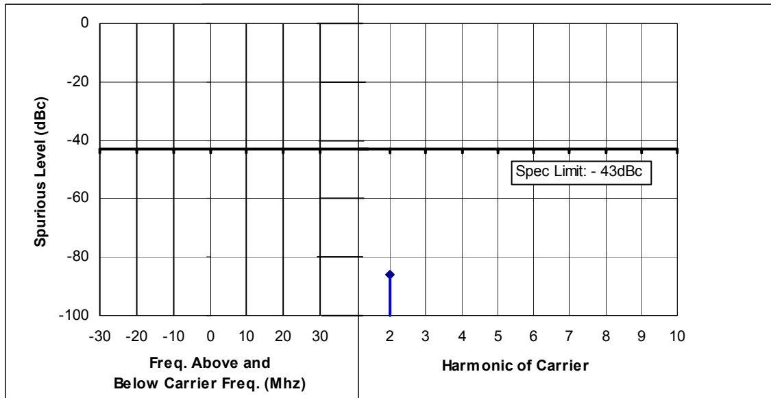
Figure 6F-11: 1 Watts, 149.00 MHz, 25 KHz Channel Spacing
