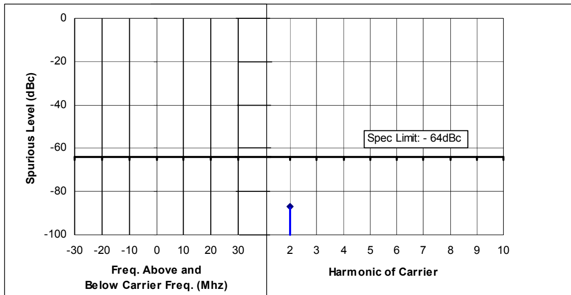
Figure 6F-2: 25 Watts, 149.00 MHz, 12.5 KHz Channel Spacing
