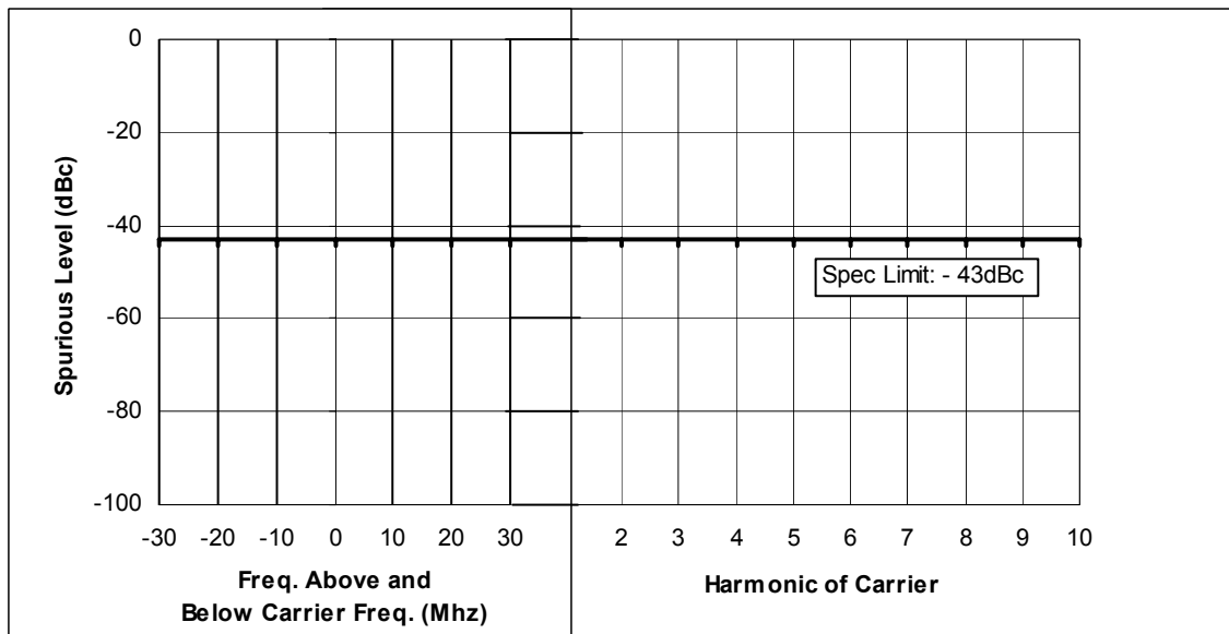
Figure 6F-12: 1 Watts, 161.75 MHz, 25 KHz Channel Spacing
