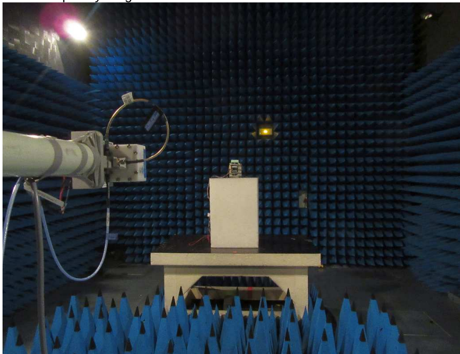
Frequency range 18 – 26.5 GHz / TPMS EWM / front side of EUT
