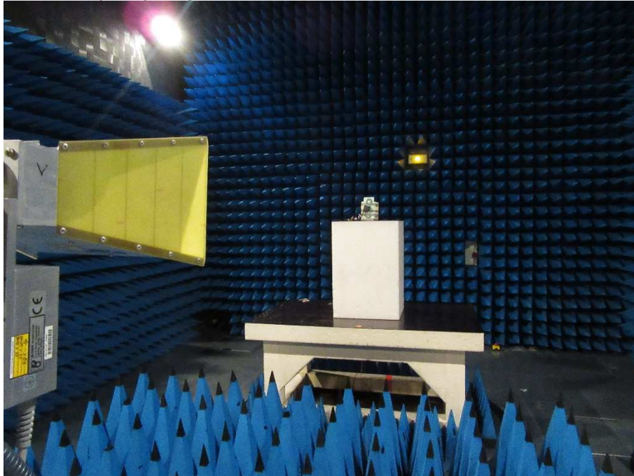
Frequency range 3 – 18 GHz / TPMS EWM / front side of EUT
