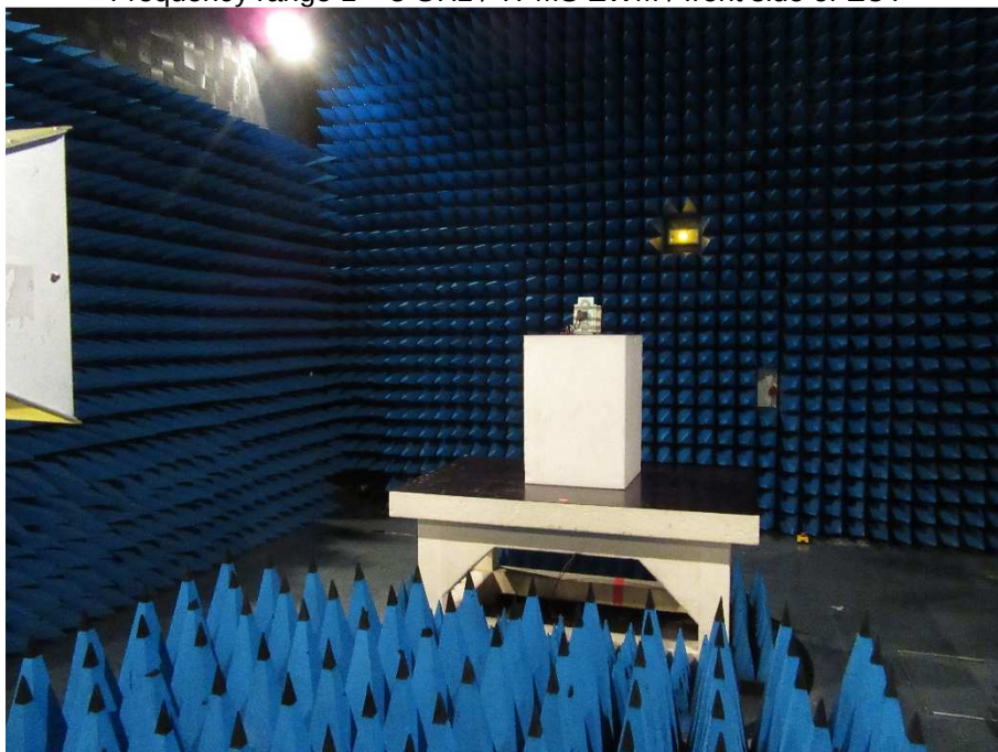
Frequency range 1 – 3 GHz / TPMS EWM / front side of EUT
