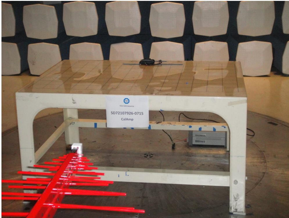
Test Setup Photo Below 1GHz Front and Back for model LMU4230CV (unintentional)
