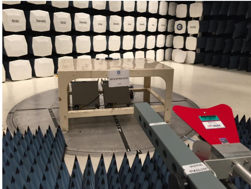
Test Setup Photo Above 1GHz Front and Back model LMU4231CV as represented sample (intentional)
