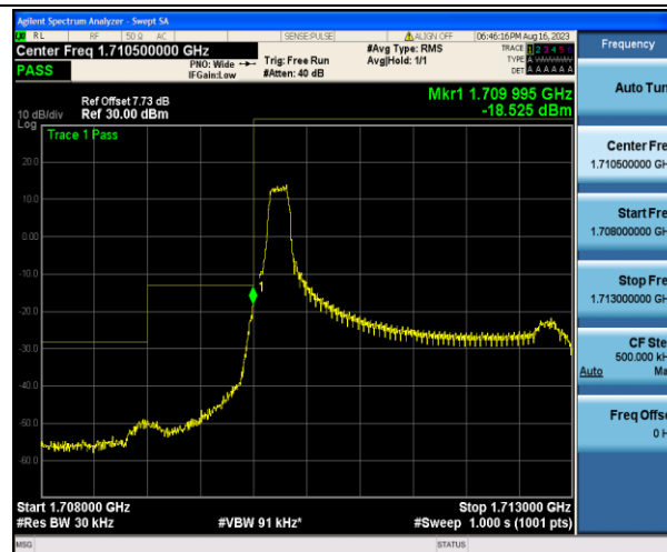
Band4_3MHz_16QAM_19965_1RB#0
