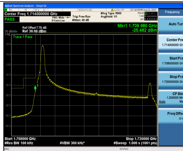
Band4_10MHz_QPSK_20000_1RB#0
