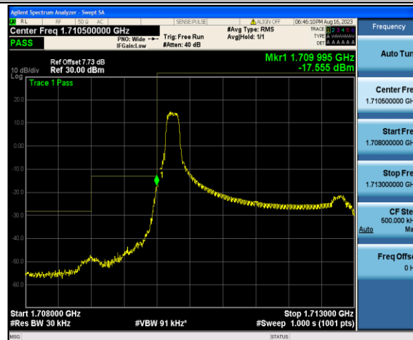
Band4_3MHz_QPSK_19965_1RB#0
