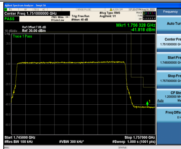
Band4_10MHz_QPSK_20350_50RB#0
