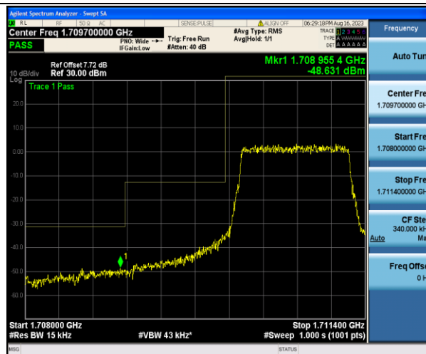
Band4_1.4MHz_16QAM_19957_6RB#0
