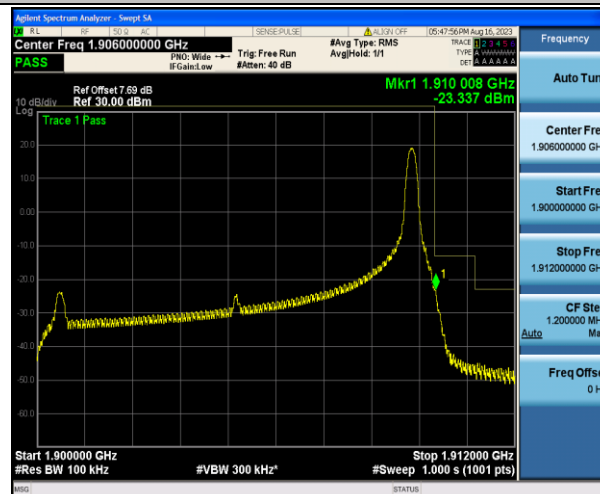
Band2_10MHz_QPSK_19150_1RB#49
