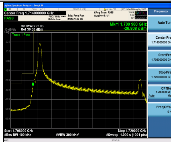
Band4_10MHz_16QAM_20000_1RB#0
