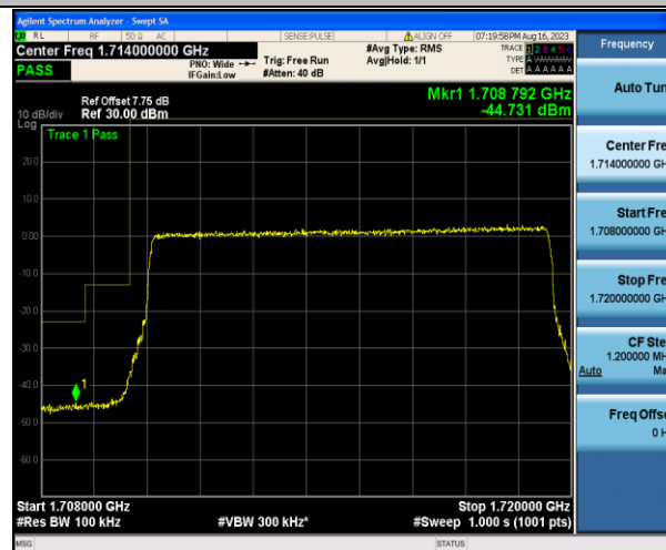
Band4_10MHz_QPSK_20000_50RB#0
