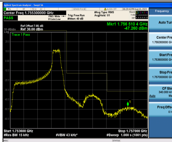
Band4_1.4MHz_16QAM_20393_1RB#5
