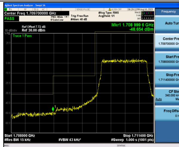
Band4_1.4MHz_QPSK_19957_6RB#0
