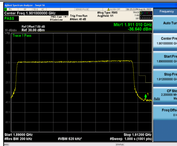
Band2_20MHz_QPSK_19100_100RB#0
