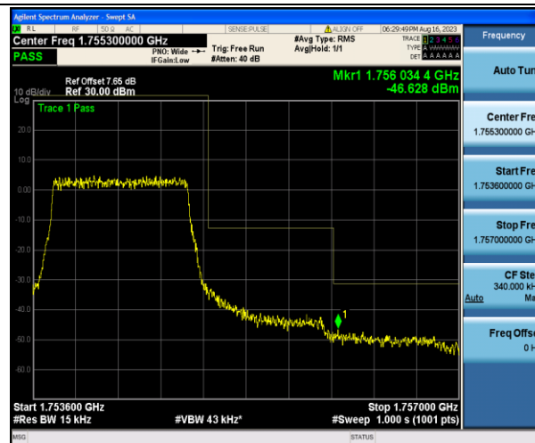
Band4_1.4MHz_QPSK_20393_6RB#0
