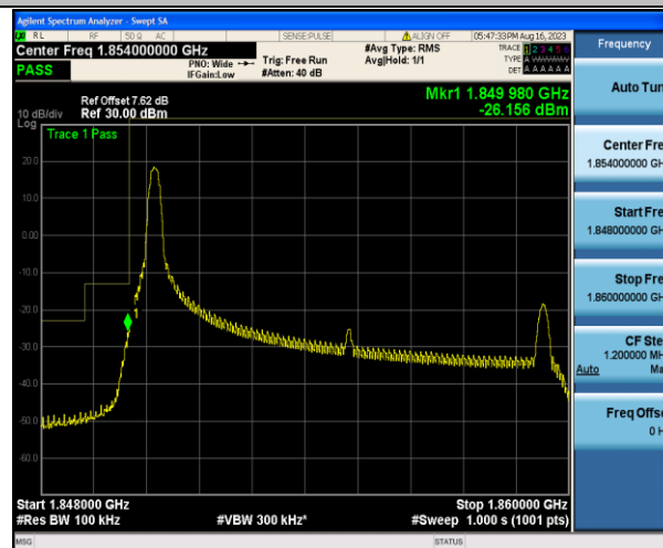
Band2_10MHz_16QAM_18650_1RB#0
