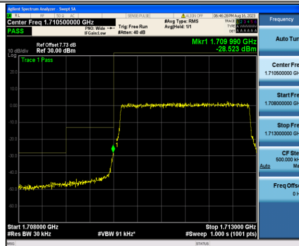
Band4_3MHz_16QAM_19965_15RB#0
