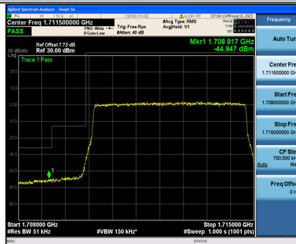
Band4_5MHz_16QAM_19975_25RB#0
