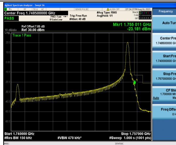
Band4_15MHz_QPSK_20325_1RB#74
