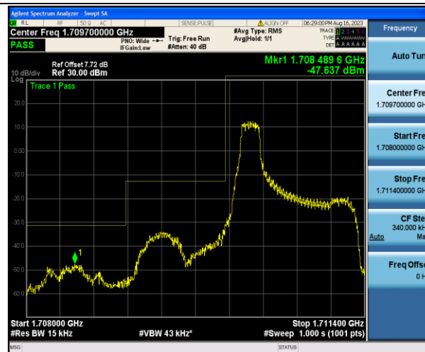
Band4_1.4MHz_QPSK_19957_1RB#0
