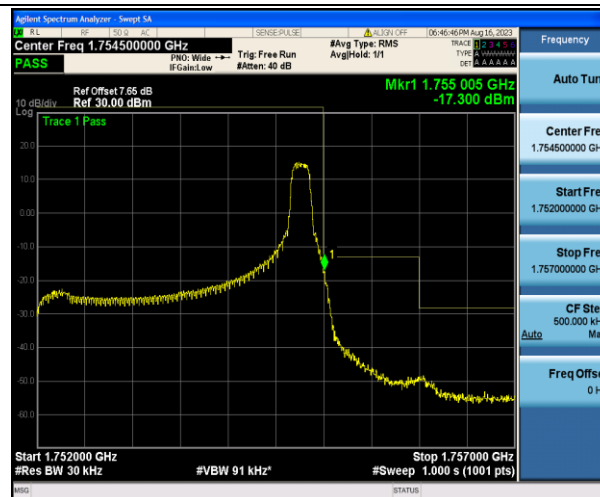
Band4_3MHz_QPSK_20385_1RB#14
