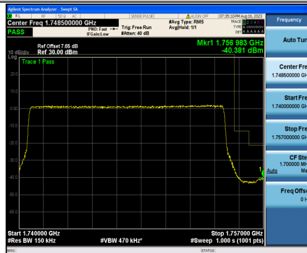
Band4_15MHz_QPSK_20325_75RB#0
