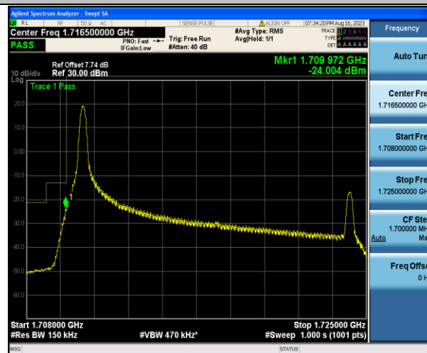
Band4_15MHz_16QAM_20025_1RB#0
