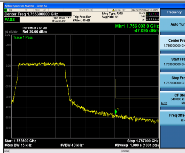
Band4_1.4MHz_16QAM_20393_6RB#0
