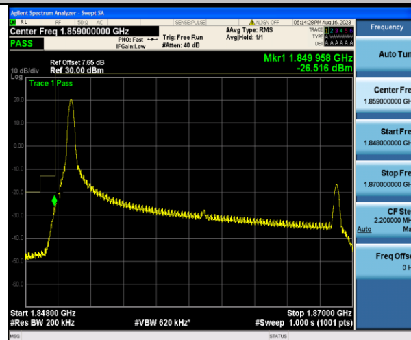
Band2_20MHz_16QAM_18700_1RB#0
