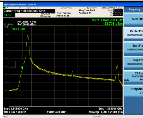
Band2_15MHz_16QAM_18675_1RB#0
