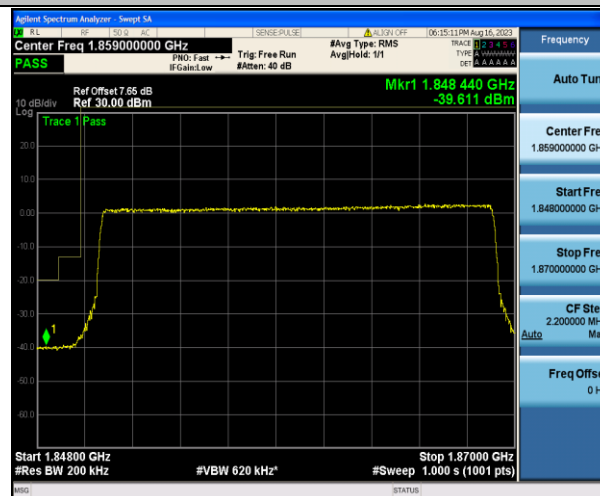
Band2_20MHz_QPSK_18700_100RB#0
