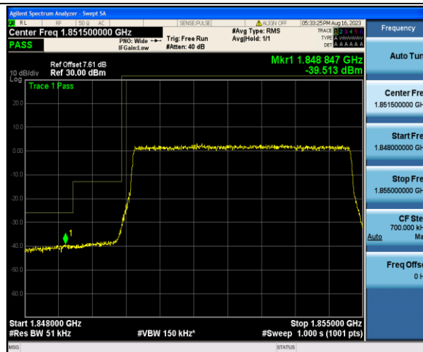
Band2_5MHz_QPSK_18625_25RB#0
