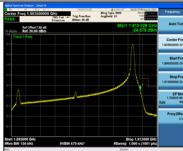
Band2_15MHz_QPSK_19125_1RB#74
