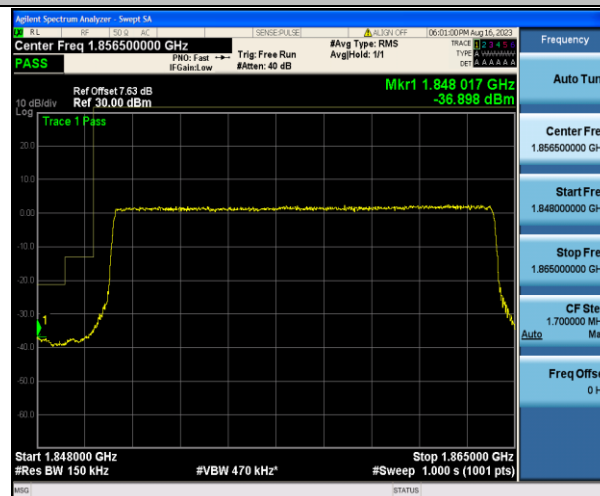
Band2_15MHz_QPSK_18675_75RB#0
