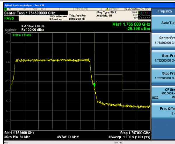
Band4_3MHz_QPSK_20385_15RB#0
