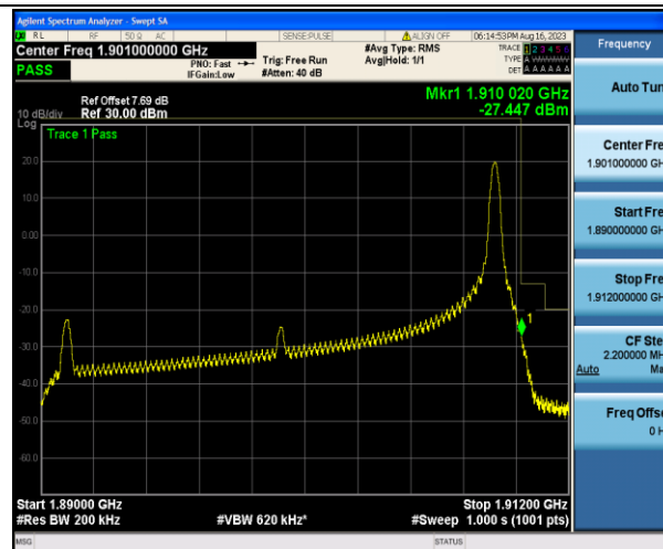
Band2_20MHz_16QAM_19100_1RB#99
