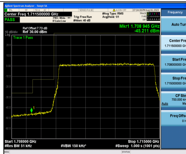
Band4_5MHz_QPSK_19975_25RB#0
