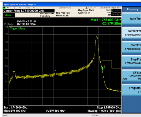
Band4_10MHz_16QAM_20350_1RB#49
