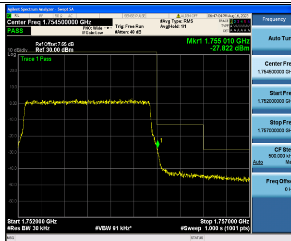
Band4_3MHz_16QAM_20385_15RB#0
