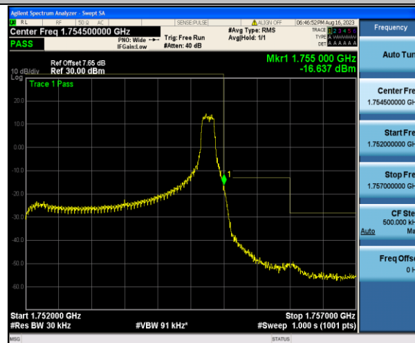
Band4_3MHz_16QAM_20385_1RB#14
