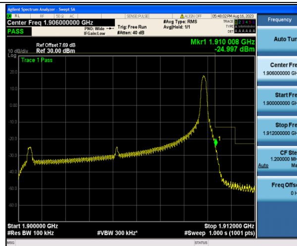
Band2_10MHz_16QAM_19150_1RB#49
