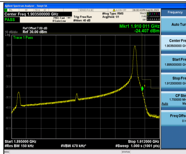
Band2_15MHz_16QAM_19125_1RB#74
