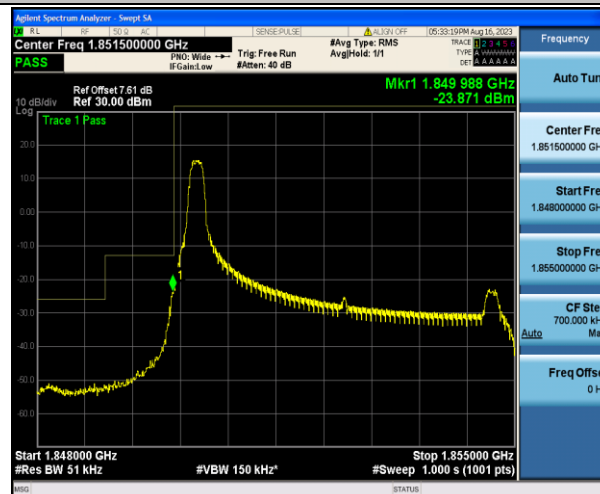
Band2_5MHz_16QAM_18625_1RB#0
