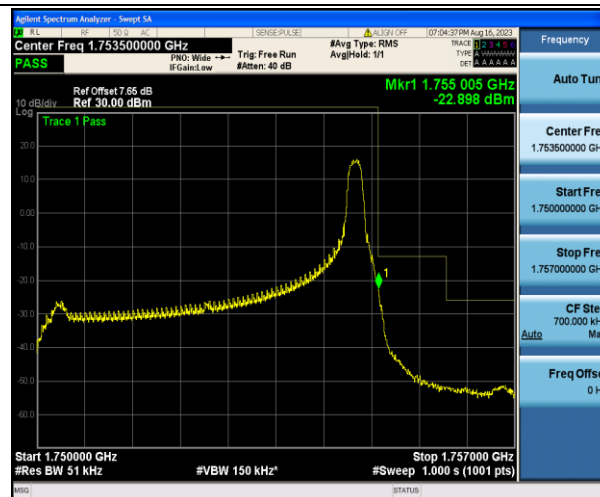
Band4_5MHz_16QAM_20375_1RB#24
