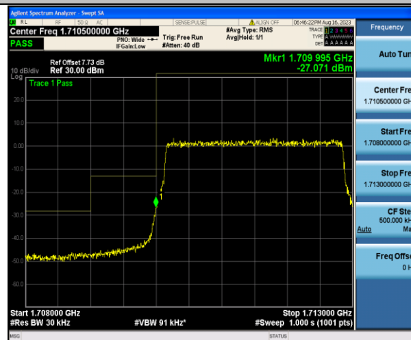
Band4_3MHz_QPSK_19965_15RB#0
