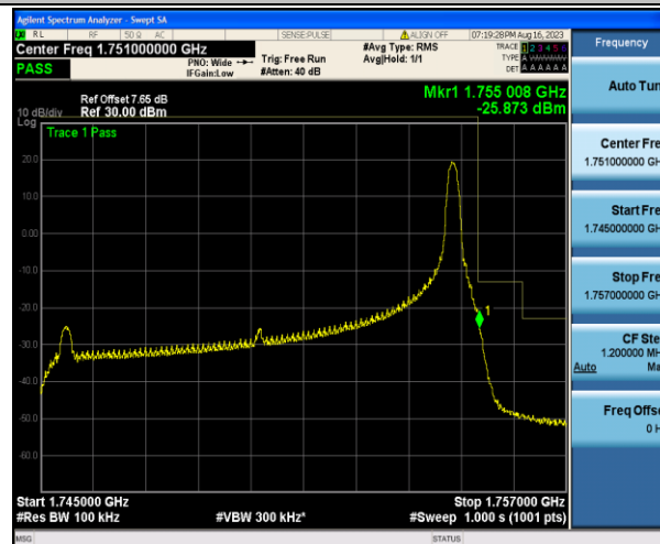
Band4_10MHz_QPSK_20350_1RB#49
