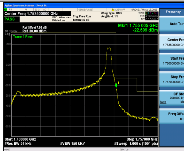
Band4_5MHz_QPSK_20375_1RB#24
