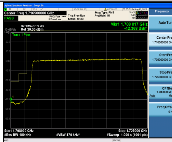
Band4_15MHz_QPSK_20025_75RB#0
