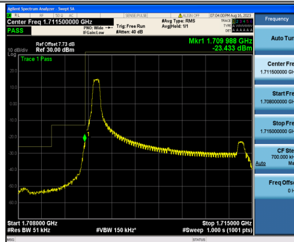
Band4_5MHz_16QAM_19975_1RB#0
