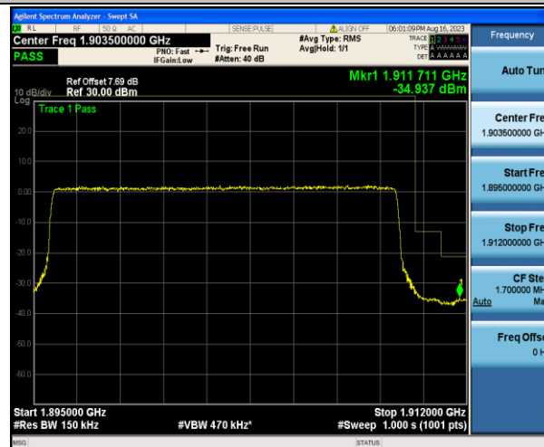
Band2_15MHz_QPSK_19125_75RB#0
