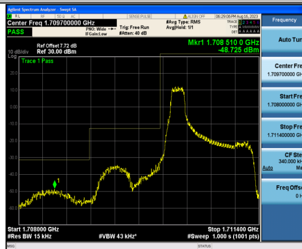
Band4_1.4MHz_16QAM_19957_1RB#0
