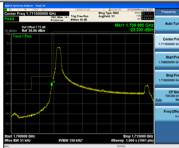
Band4_5MHz_QPSK_19975_1RB#0
