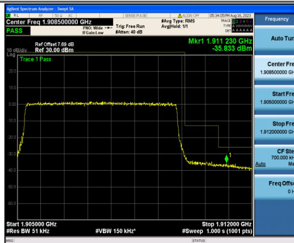
Band2_5MHz_16QAM_19175_25RB#0
