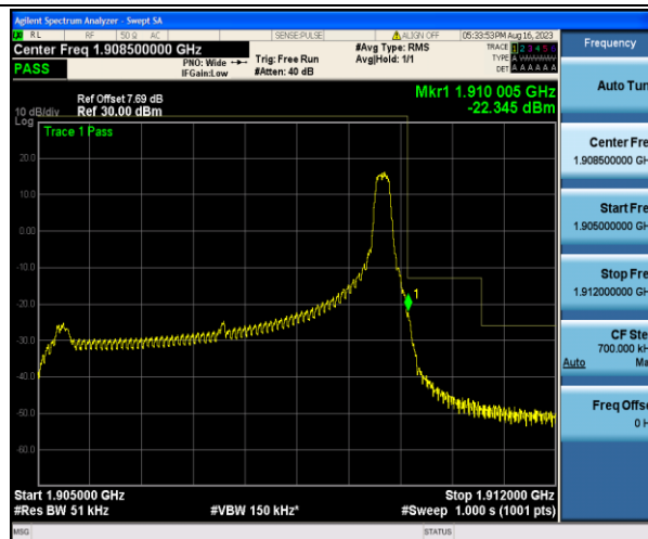
Band2_5MHz_16QAM_19175_1RB#24
