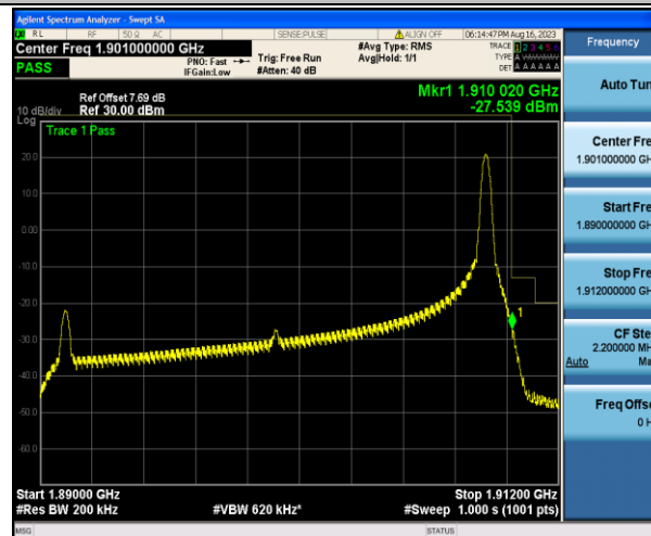
Band2_20MHz_QPSK_19100_1RB#99
