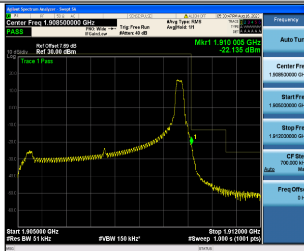
Band2_5MHz_QPSK_19175_1RB#24
