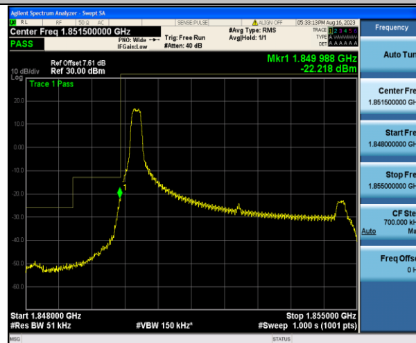
Band2_5MHz_QPSK_18625_1RB#0
