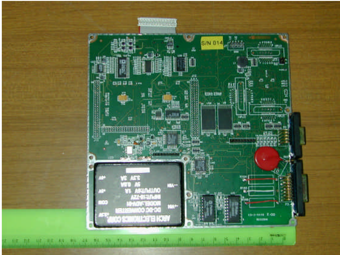
FCC ID:PIDMARCONI; SPR-2.4 main board front view
