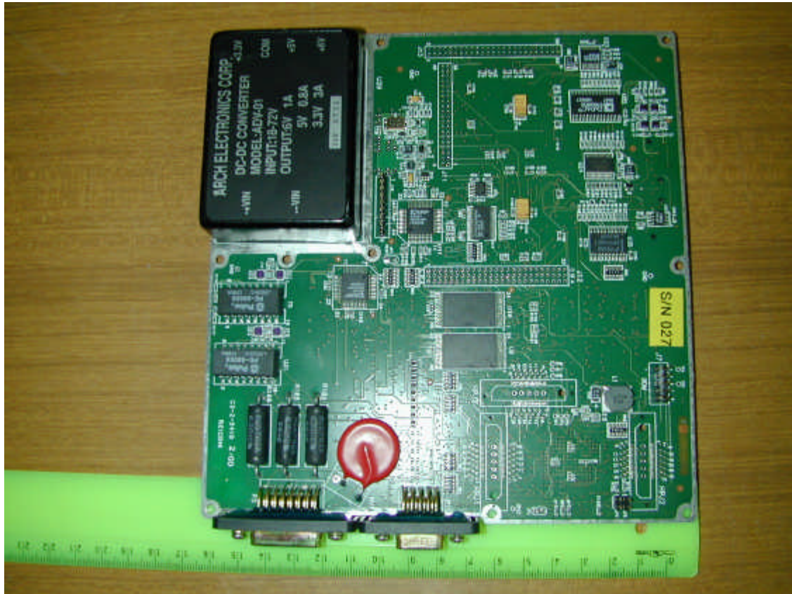
FCC ID:PIDMARCONI; BSR-2.4 main board front view
