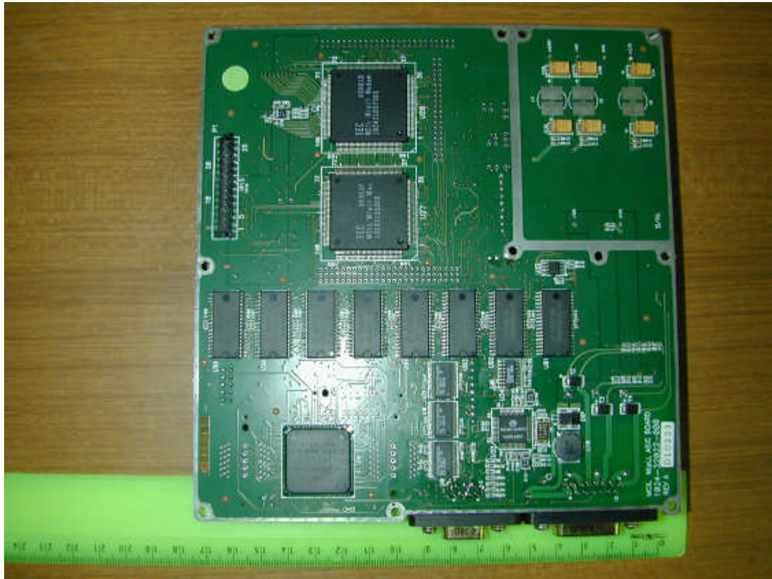
FCC ID:PIDMARCONI; BSR-2.4 main board rear view
