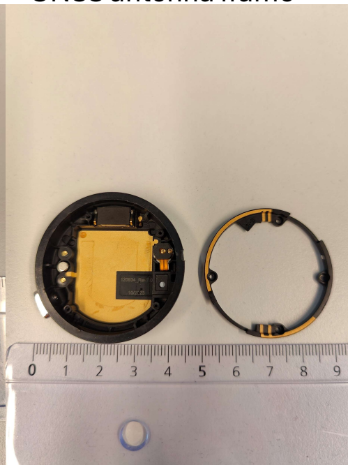
LTE Antenna and BT & GNSS antenna frame
