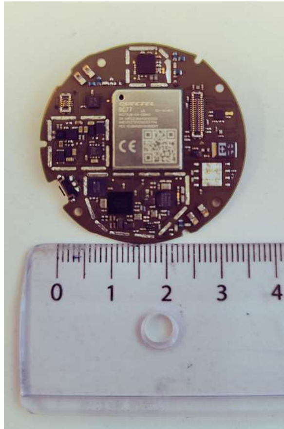
PCB top without RF shields
