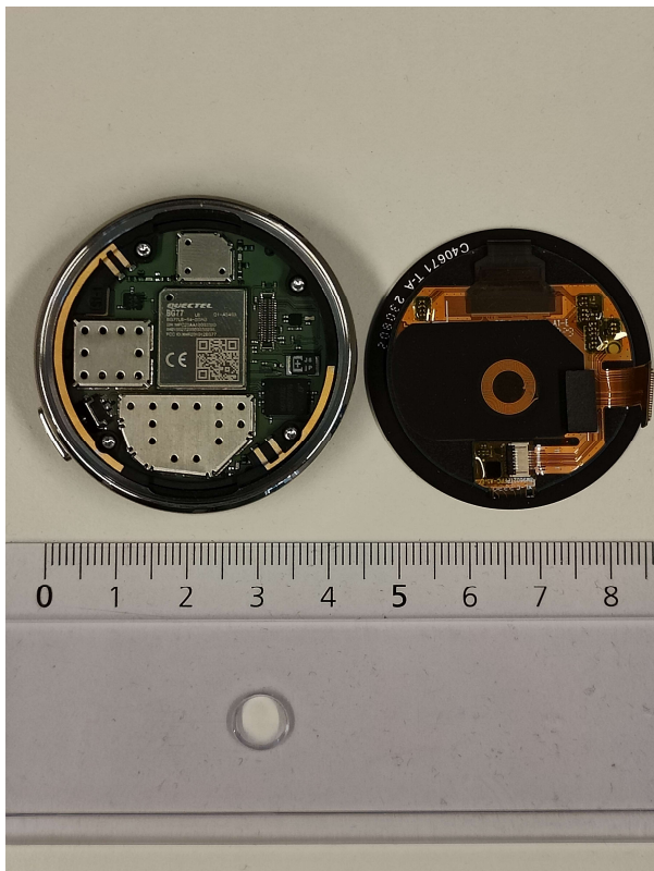
Frontview inside
