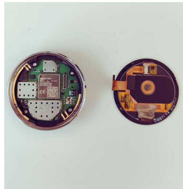
Connector disconnected
