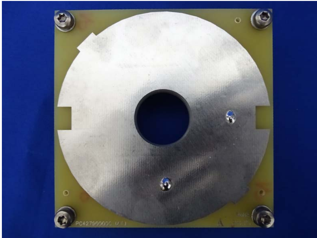
(20) EUT Photo-Antenna
