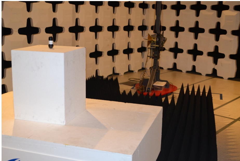
Radiated Emissions 1 – 18 GHz
