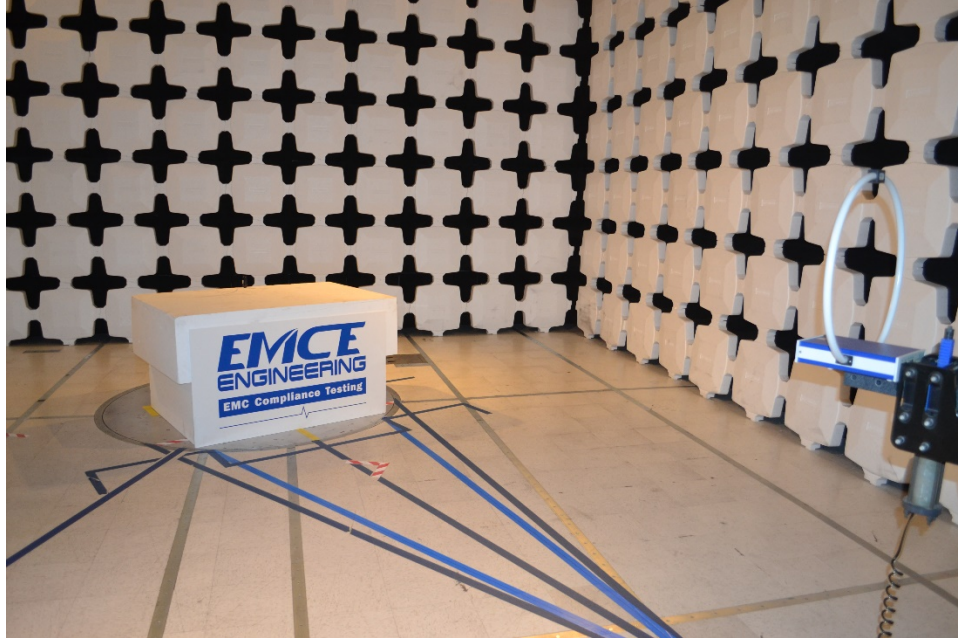
Radiated Emissions <30 MHz
