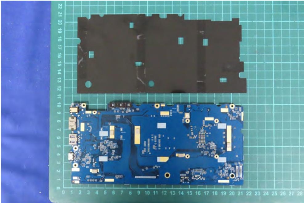
(27) EUT Photo
