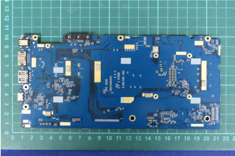
(28) EUT Photo
