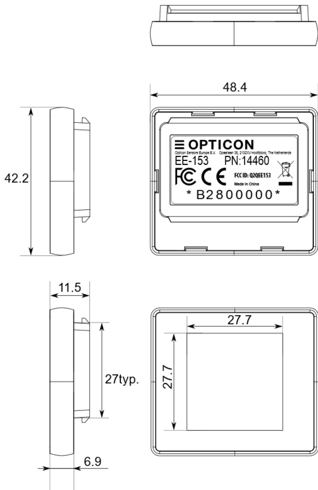
Figure 8: Mechanical drawing
