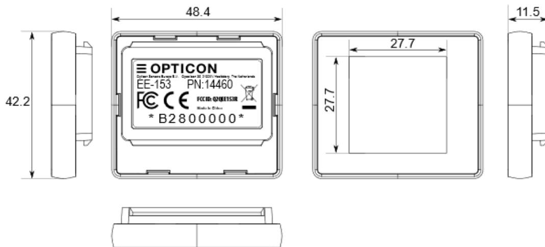
Figure 1: Dimensions
