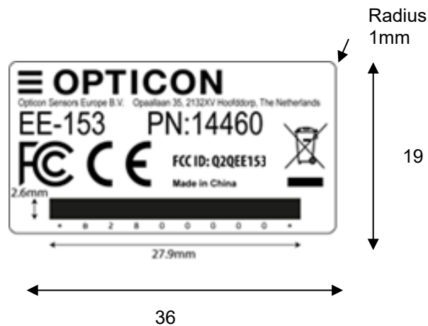
Figure 3: Product Label dimensions
