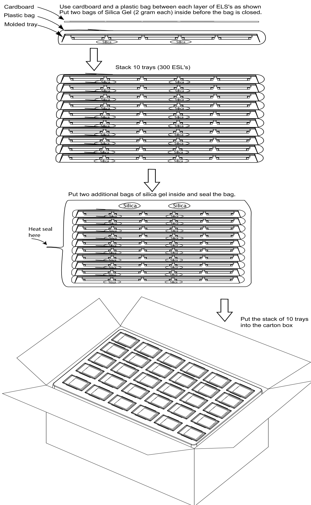
Figure 6: collective packaging
