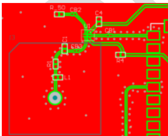
GPS Layout
