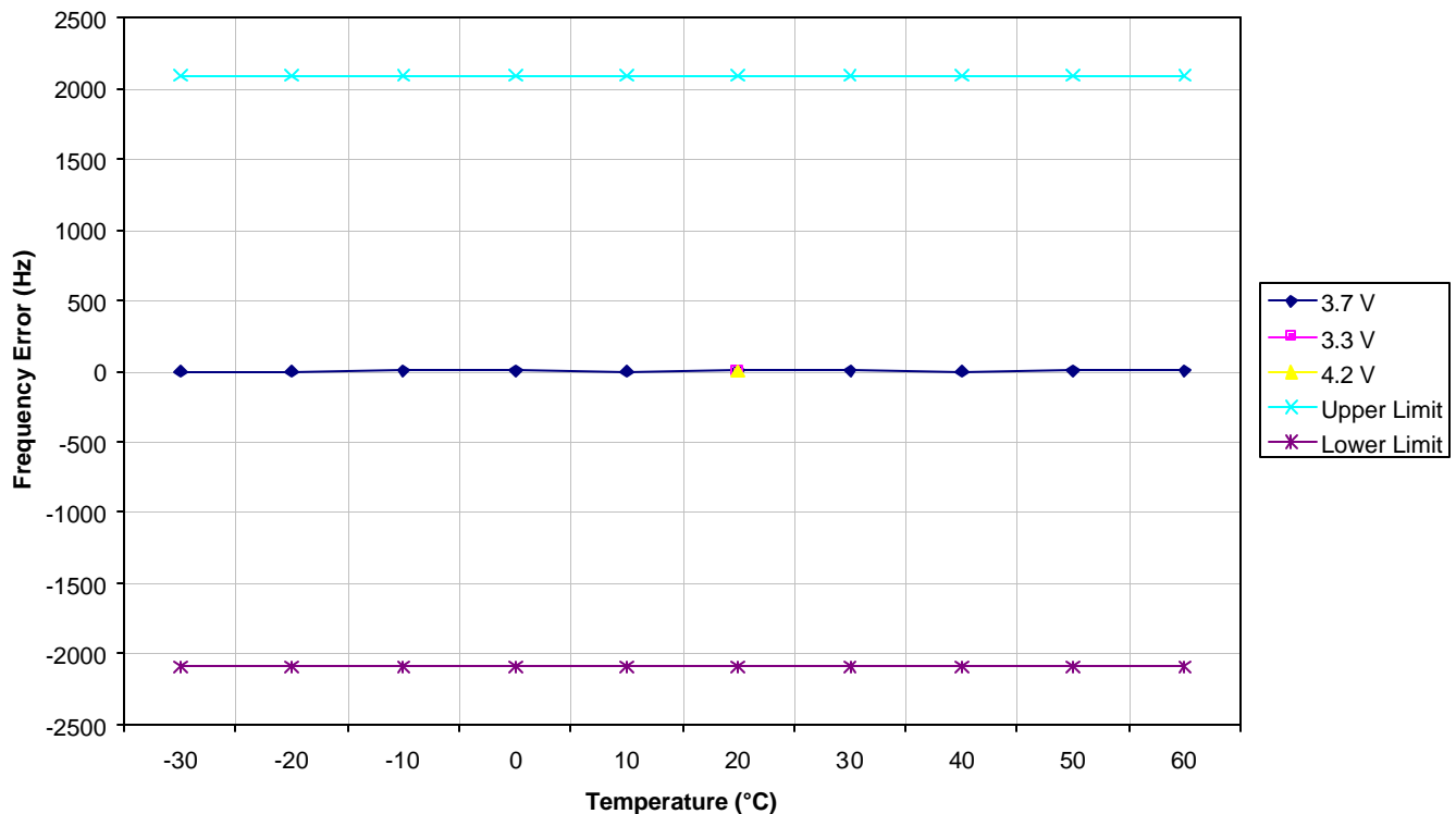
OVFKWC-KX17 CDMA 800 MHz Transmit RF Carrier Stability Over Temperature and Voltage
