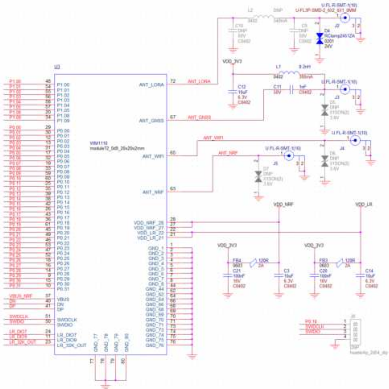
Figure 6 Reference design based on WM1110
