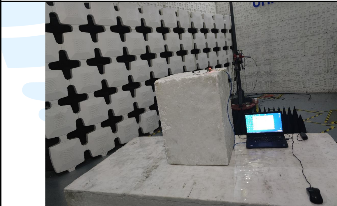
Radiated emission Test Setup (Above 1 GHz) _Right earbuds
