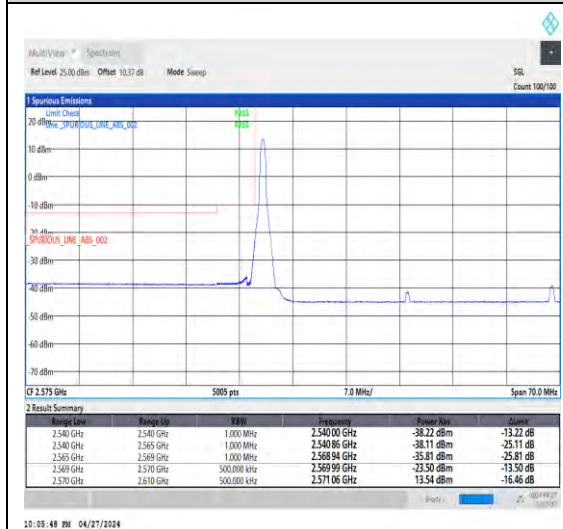
1-N38-30-40-L-4-CP-QPSK-Edge_1RB_Left-1@0-Ant1-1--PASS-see graph
