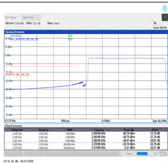
1-N38-30-30-L-6-CP-QPSK-Outer_Full-78@0-Ant1-1--PASS-see graph
