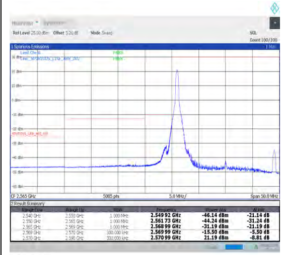
1-N38--30-20-L-4-CP-QPSK-Edge_1RB_Left-1@0-Ant1-1--PASS-see graph
