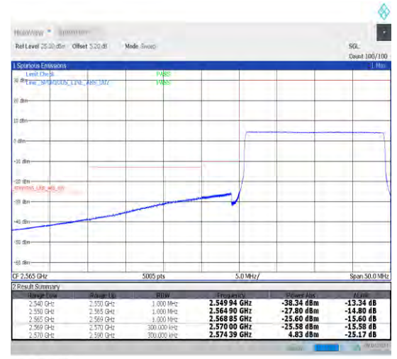
1-N38--30-20-L-6-CP-QPSK-Outer_Full-51@0-Ant1-1--PASS-see graph
