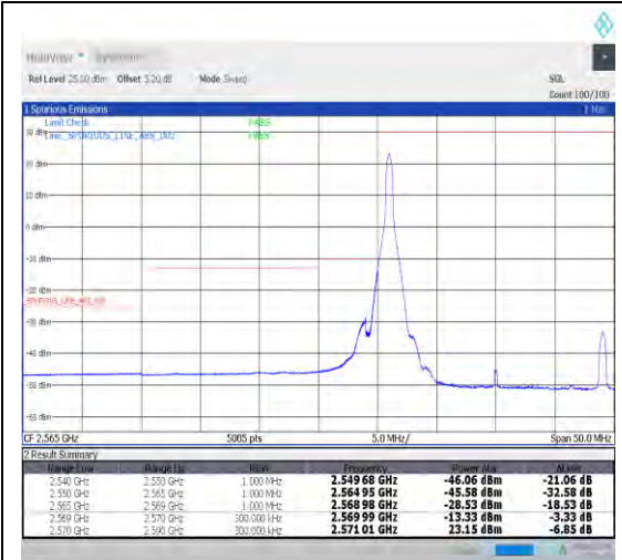
1-N38--30-20-L-1-DFT-PI2BPSK-Edge_1RB_Left-1@0-Ant1-1--PASS-see graph
