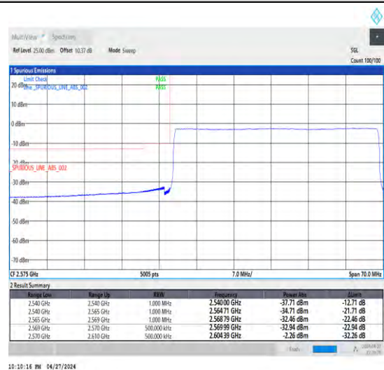
1-N38-30-40-L-6-CP-QPSK-Outer_Full-106@0-Ant1-1--PASS-see graph
