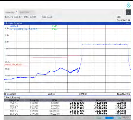
1-N38--30-20-L-3-DFT-PI2BPSK-Outer_Full-50@0-Ant1-1--PASS-see graph
