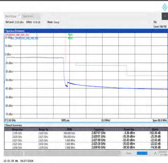
1-N38-30-30-H-6-CP-QPSK-Outer_Full-78@0-Ant1-1--PASS-see graph
