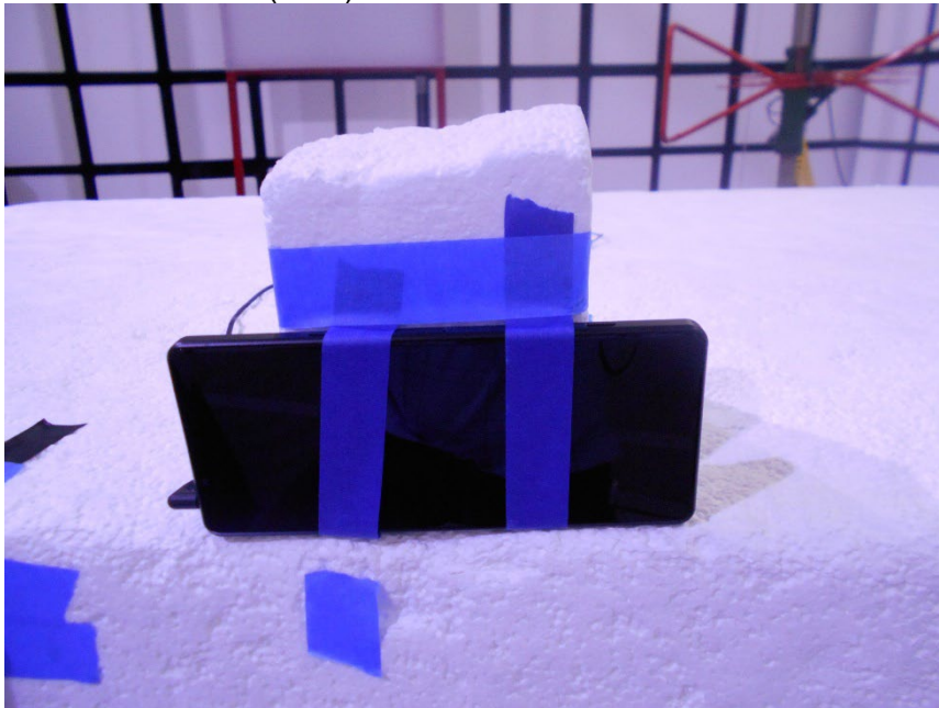
Y-ORIENTATION (NFC)
