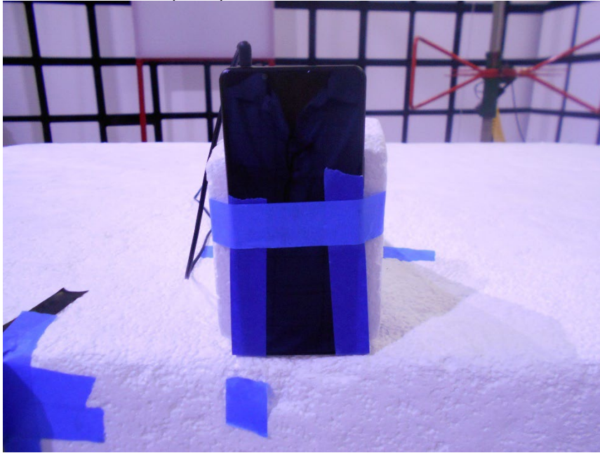
Z-ORIENTATION (NFC)
