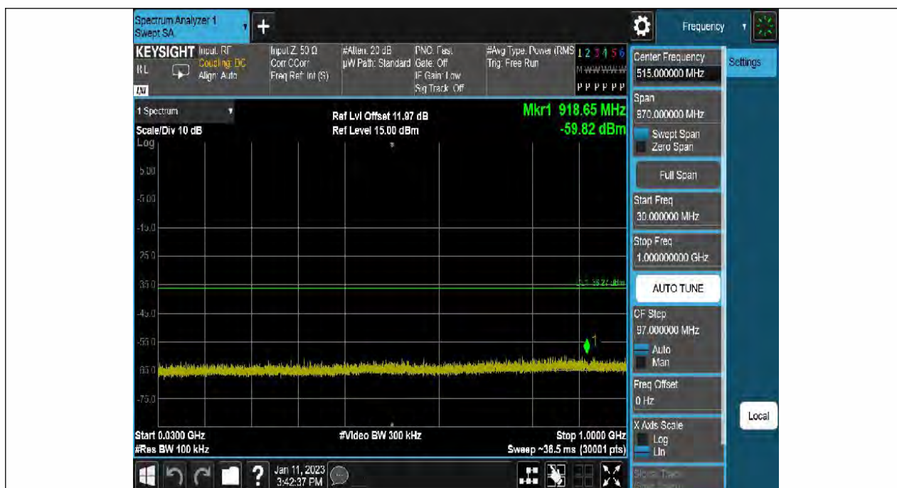
11N40SISO-Ant1-2452-30~1000--6.27
