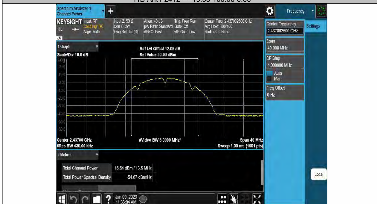
11B-Ant1-2437-----16.64-100.00-0.00
