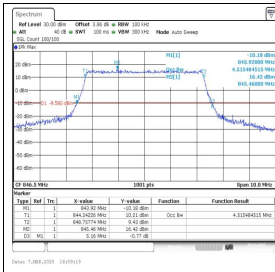
26(824-849)-5MHz-QPSK-27015-25RB#0-PASS
