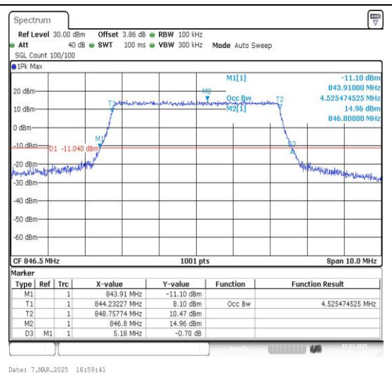
26(824-849)-5MHz-16QAM-27015-25RB#0-PASS
