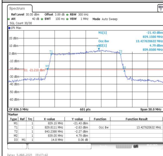
26(824-849)-15MHz-QPSK-26915-75RB#0-PASS
