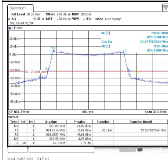
26(824-849)-15MHz-QPSK-26865-75RB#0-PASS
