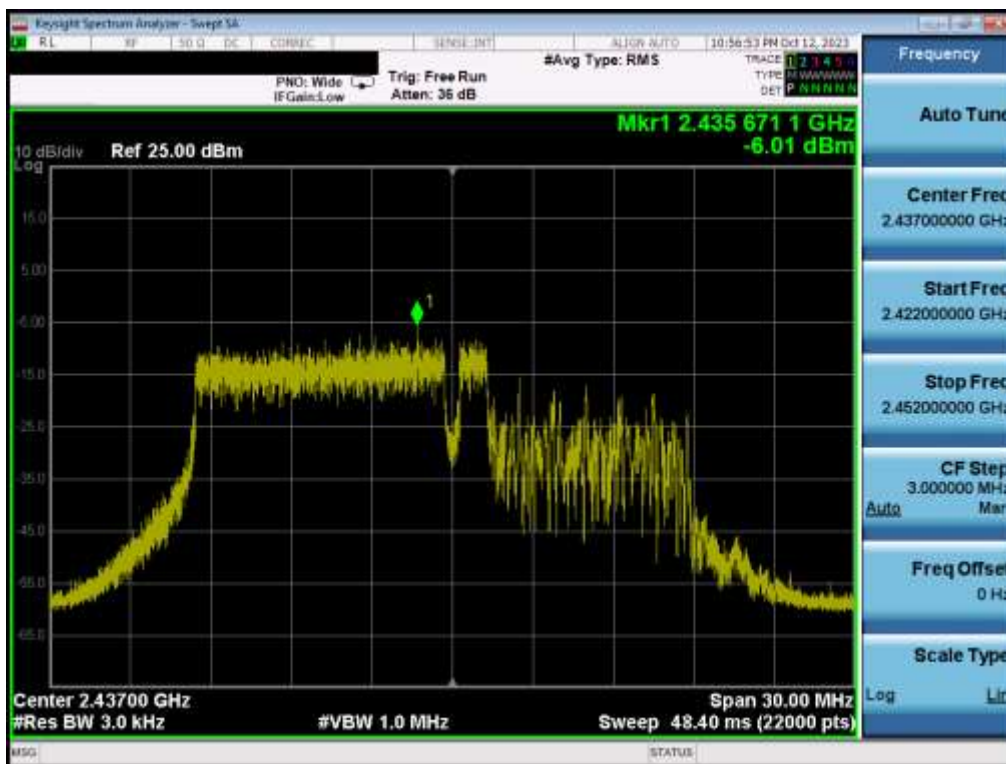
Plot 7-28. Power Spectral Density Plot MIMO ANT2 (802.11be OFDMA – 106 + 26 Tones – Ch. 6)
