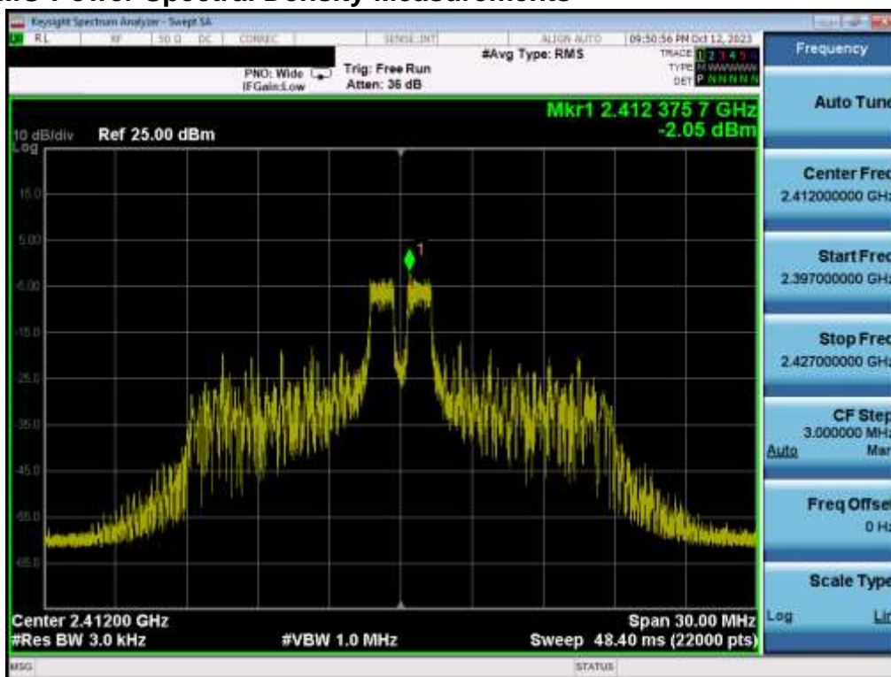
Plot 7-13. Power Spectral Density Plot MIMO ANT1 (802.11be OFDMA – 26 Tones – Ch. 1)
