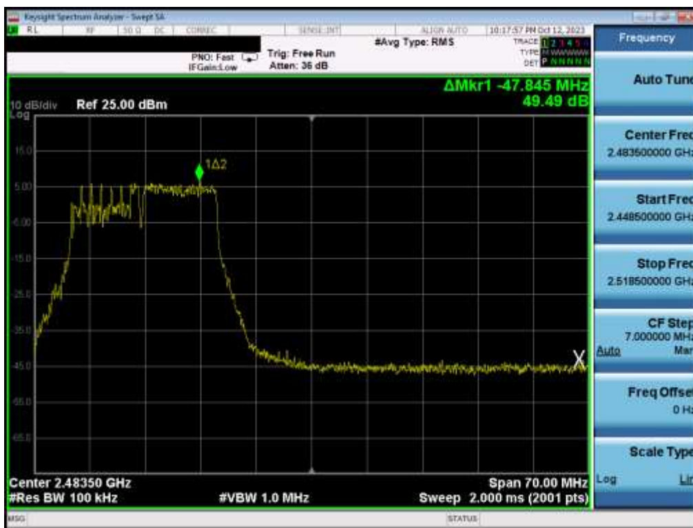
Plot 7-32. Band Edge Plot MIMO ANT1 (802.11be OFDMA – 106 + 26 Tones – Ch. 11)
