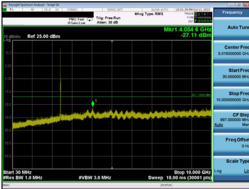
Plot 7-67. Conducted Spurious Plot MIMO ANT2 (802.11be OFDMA – 26 Tones – Ch. 6)
