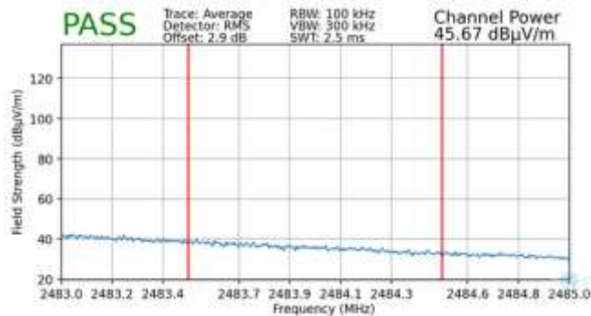
Plot 7-91. Radiated Restricted Upper Band Edge Measurement MIMO (Average – 106 + 26 Tones)
