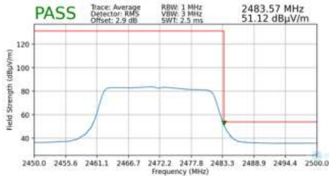
Plot 7-99. Radiated Restricted Upper Band Edge Measurement MIMO (Average – 242 Tones)
