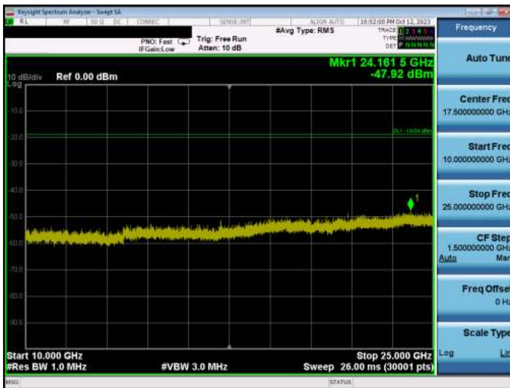
Plot 7-68. Conducted Spurious Plot MIMO ANT2 (802.11be OFDMA – 26 Tones – Ch. 6)
