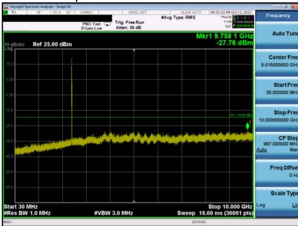
Plot 7-53. Conducted Spurious Plot MIMO ANT1 (802.11be OFDMA – 26 Tones – Ch. 1)
