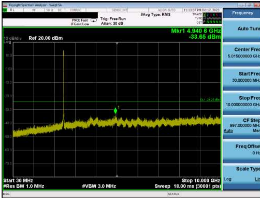
Plot 7-75. Conducted Spurious Plot MIMO ANT2 (802.11be OFDMA – 242 Tones – Ch. 11)
