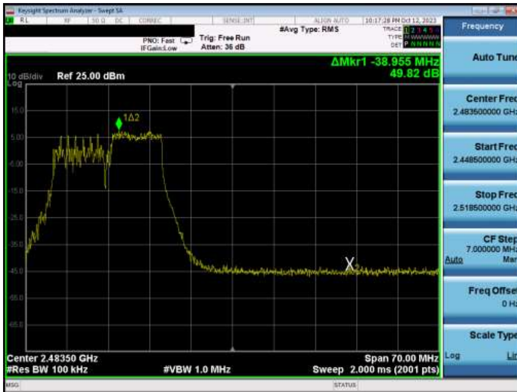
Plot 7-31. Band Edge Plot MIMO ANT1 (802.11be OFDMA – 106 Tones – Ch. 11)
