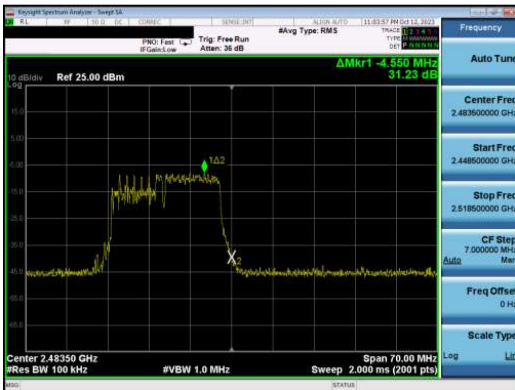
Plot 7-48. Band Edge Plot MIMO ANT2 (802.11be OFDMA – 106 + 26 Tones – Ch. 13)
