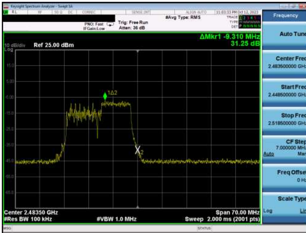
Plot 7-47. Band Edge Plot MIMO ANT2 (802.11be OFDMA – 106 Tones – Ch. 13)
