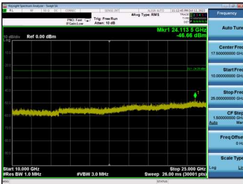
Plot 7-72. Conducted Spurious Plot MIMO ANT2 (802.11be OFDMA – 242 Tones – Ch. 1)
