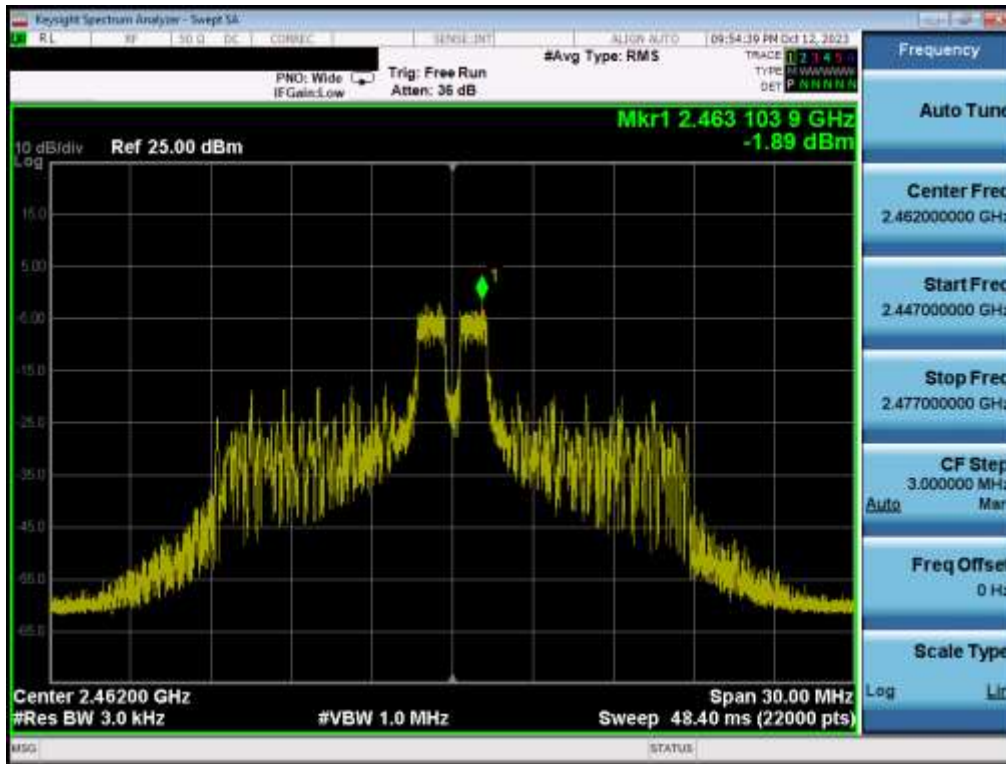
Plot 7-15. Power Spectral Density Plot MIMO ANT1 (802.11be OFDMA – 26 Tones – Ch. 11)
