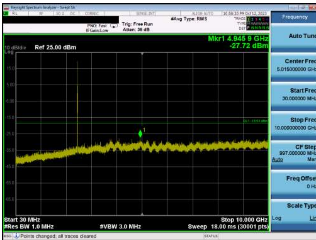
Plot 7-69. Conducted Spurious Plot MIMO ANT2 (802.11be OFDMA – 26 Tones – Ch. 11)
