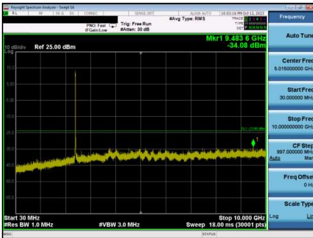
Plot 7-59. Conducted Spurious Plot MIMO ANT1 (802.11be OFDMA – 242 Tones – Ch. 1)
