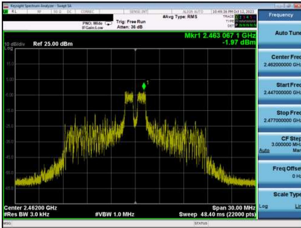
Plot 7-23. Power Spectral Density Plot MIMO ANT2 (802.11be OFDMA – 26 Tones – Ch. 11)
