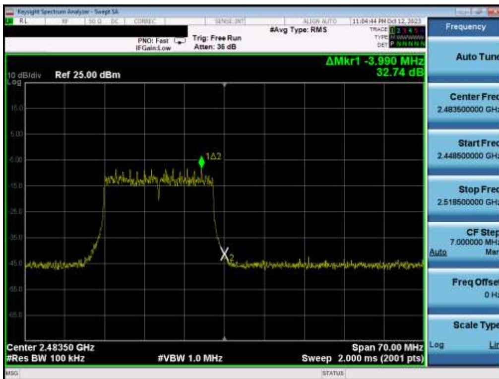
Plot 7-52. Band Edge Plot MIMO ANT2 (802.11be OFDMA - 242 Tones - Ch. 13)
