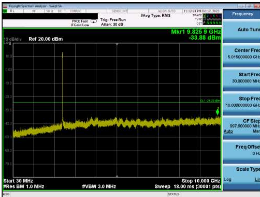
Plot 7-71. Conducted Spurious Plot MIMO ANT2 (802.11be OFDMA – 242 Tones – Ch. 1)
