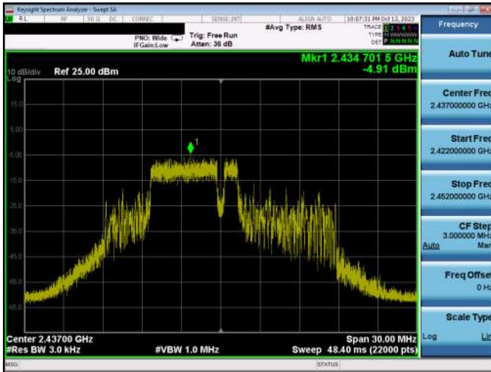
Plot 7-19. Power Spectral Density Plot MIMO ANT1 (802.11be OFDMA – 52 + 26 Tones – Ch. 6)
