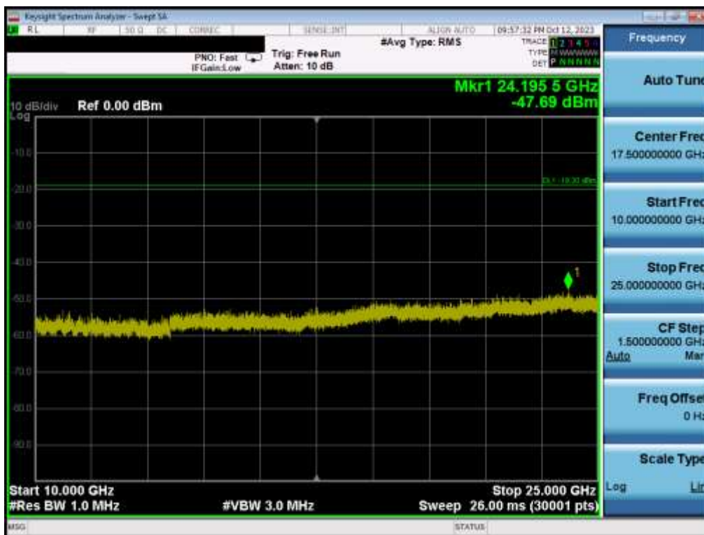
Plot 7-56. Conducted Spurious Plot MIMO ANT1 (802.11be OFDMA – 26 Tones – Ch. 6)
