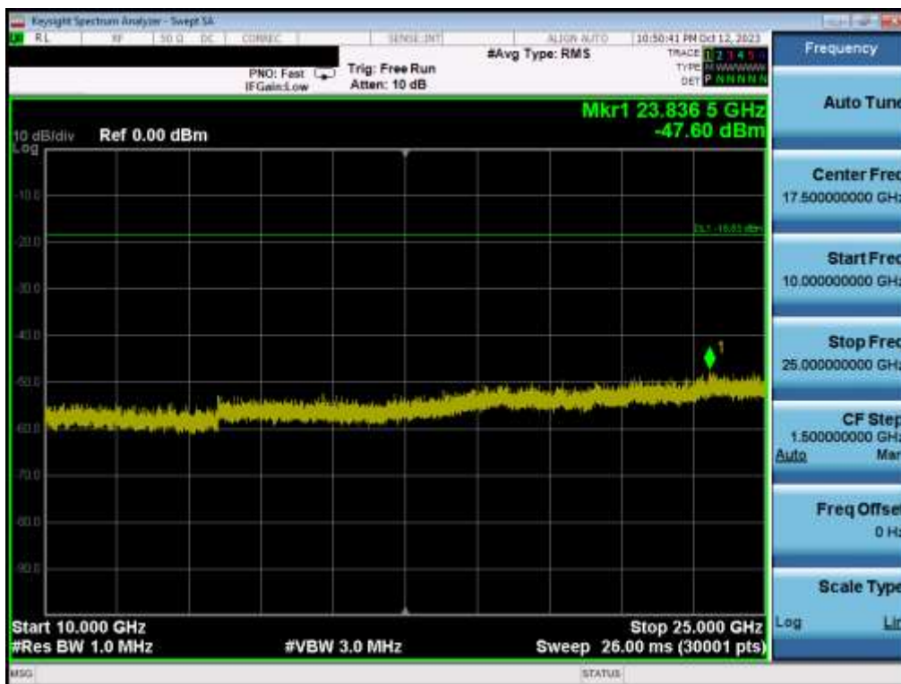
Plot 7-70. Conducted Spurious Plot MIMO ANT2 (802.11be OFDMA – 26 Tones – Ch. 11)
