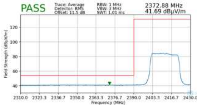
Plot 7-93. Radiated Restricted Lower Band Edge Measurement MIMO (Average – 242 Tones)
