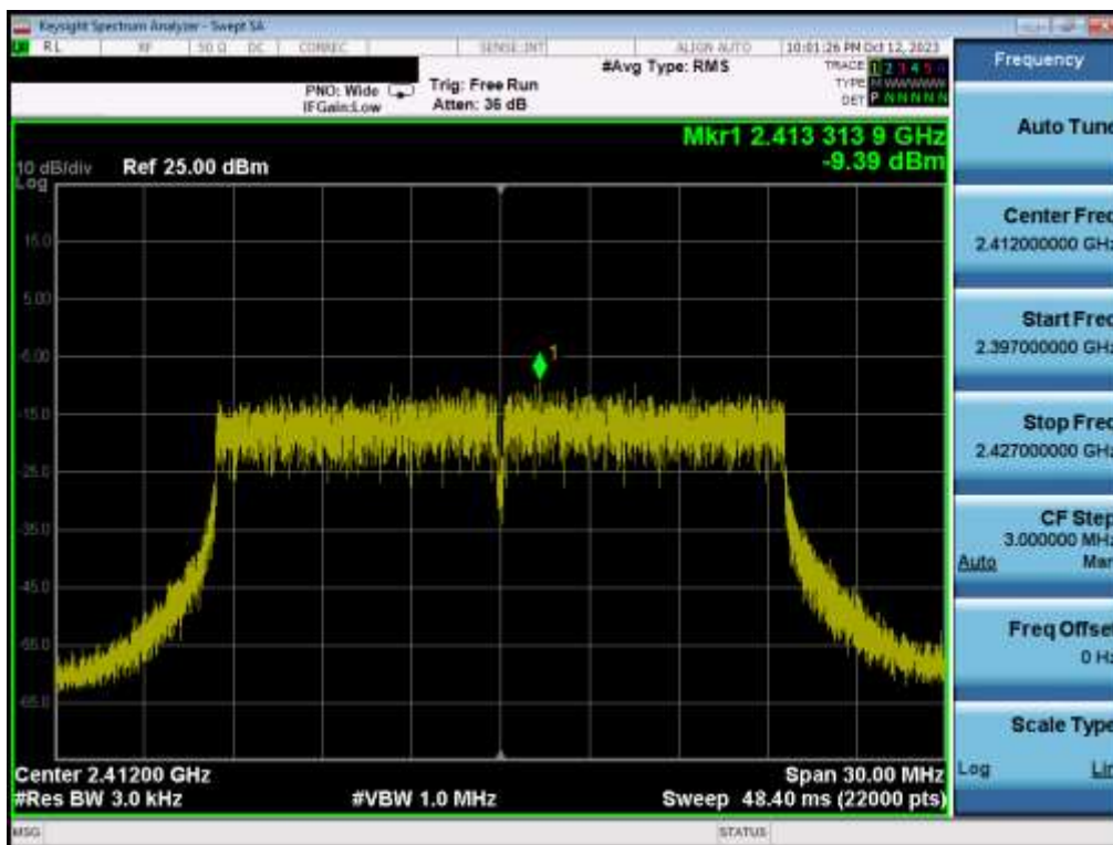
Plot 7-16. Power Spectral Density Plot MIMO ANT1 (802.11be OFDMA – 242 Tones – Ch. 1)
