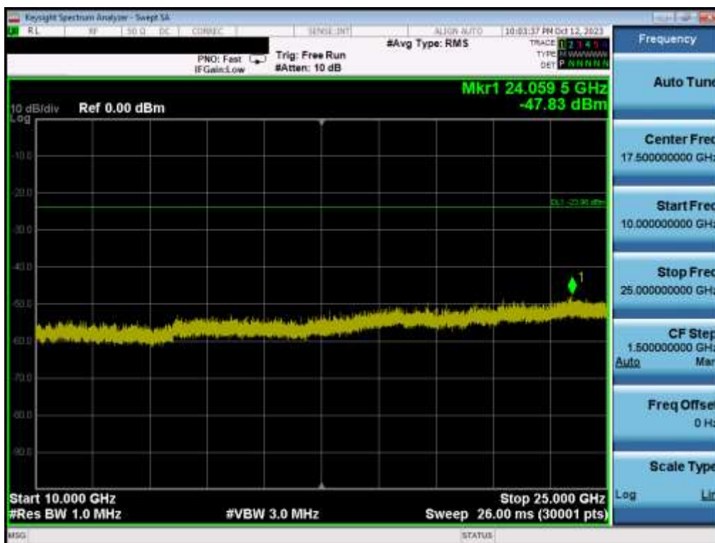
Plot 7-60. Conducted Spurious Plot MIMO ANT1 (802.11be OFDMA – 242 Tones – Ch. 1)
