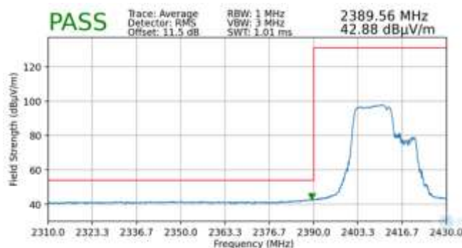
Plot 7-85. Radiated Restricted Lower Band Edge Measurement MIMO (Average – 106 + 26 Tones)
