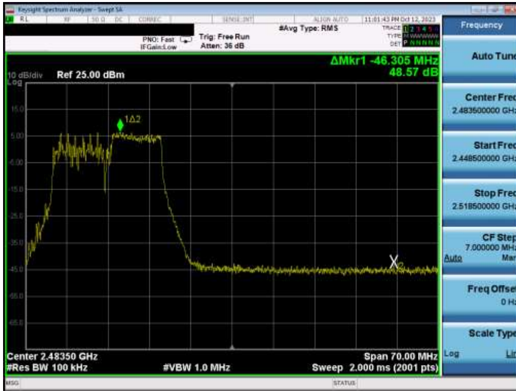
Plot 7-43. Band Edge Plot MIMO ANT2 (802.11be OFDMA – 106 Tones – Ch. 11)
