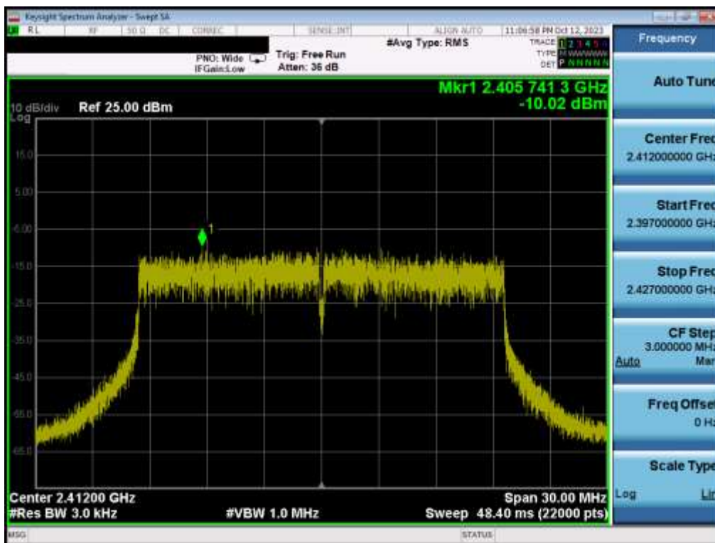
Plot 7-24. Power Spectral Density Plot MIMO ANT2 (802.11be OFDMA – 242 Tones – Ch. 1)
