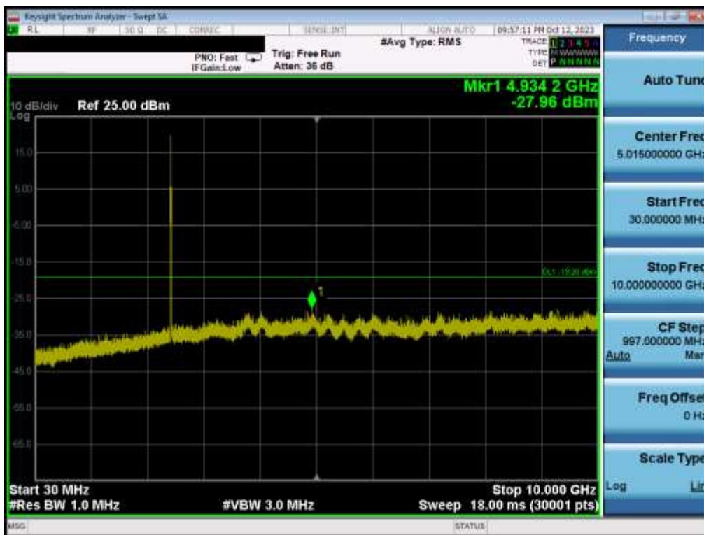
Plot 7-55. Conducted Spurious Plot MIMO ANT1 (802.11be OFDMA – 26 Tones – Ch. 6)
