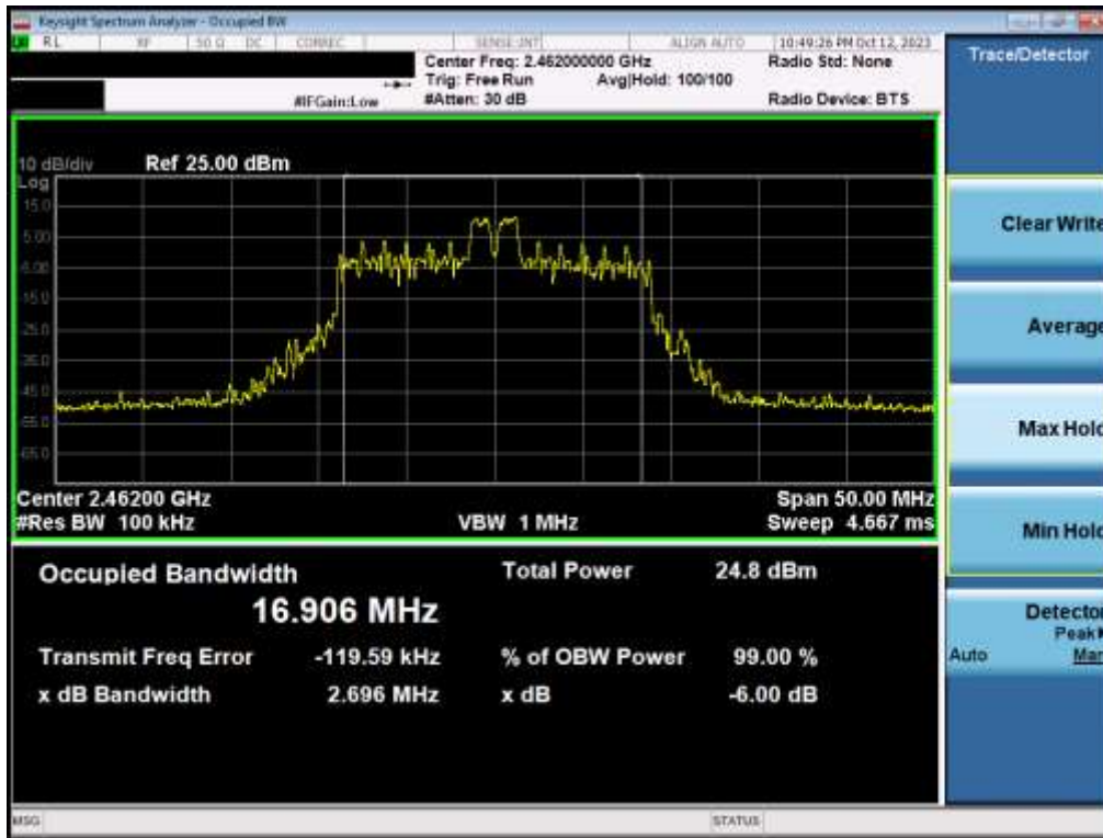
Plot 7-9. 6dB Bandwidth Plot MIMO ANT2 (802.11be OFDMA – 26 Tones – Ch. 11)
