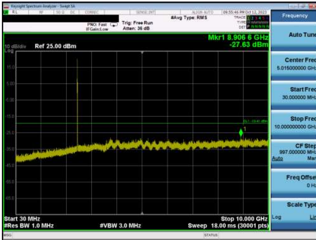
Plot 7-57. Conducted Spurious Plot MIMO ANT1 (802.11be OFDMA – 26 Tones – Ch. 11)
