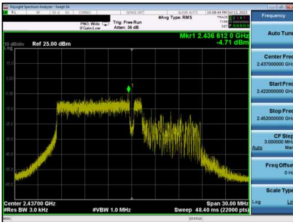
Plot 7-20. Power Spectral Density Plot MIMO ANT1 (802.11be OFDMA – 106 + 26 Tones – Ch. 6)
