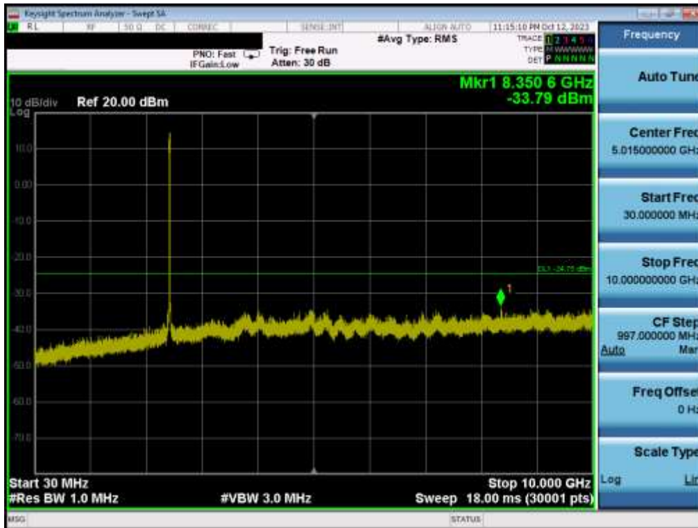
Plot 7-73. Conducted Spurious Plot MIMO ANT2 (802.11be OFDMA – 242 Tones – Ch. 6)
