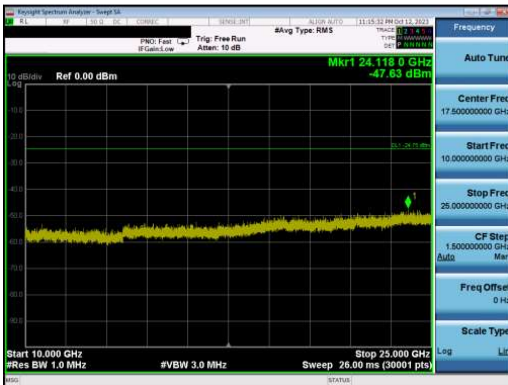
Plot 7-74. Conducted Spurious Plot MIMO ANT2 (802.11be OFDMA – 242 Tones – Ch. 6)
