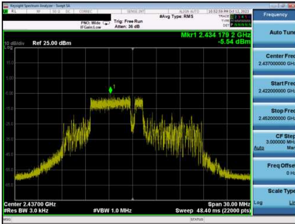
Plot 7-27. Power Spectral Density Plot MIMO ANT2 (802.11be OFDMA – 52 + 26 Tones – Ch. 6)
