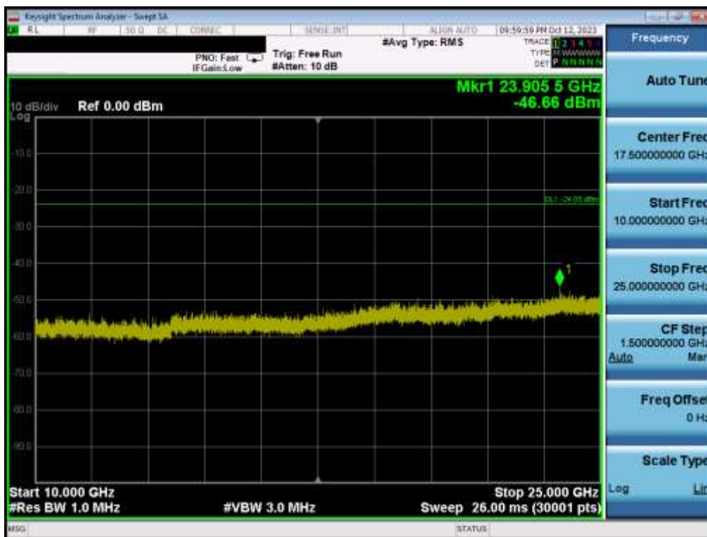
Plot 7-62. Conducted Spurious Plot MIMO ANT1 (802.11be OFDMA – 242 Tones – Ch. 6)
