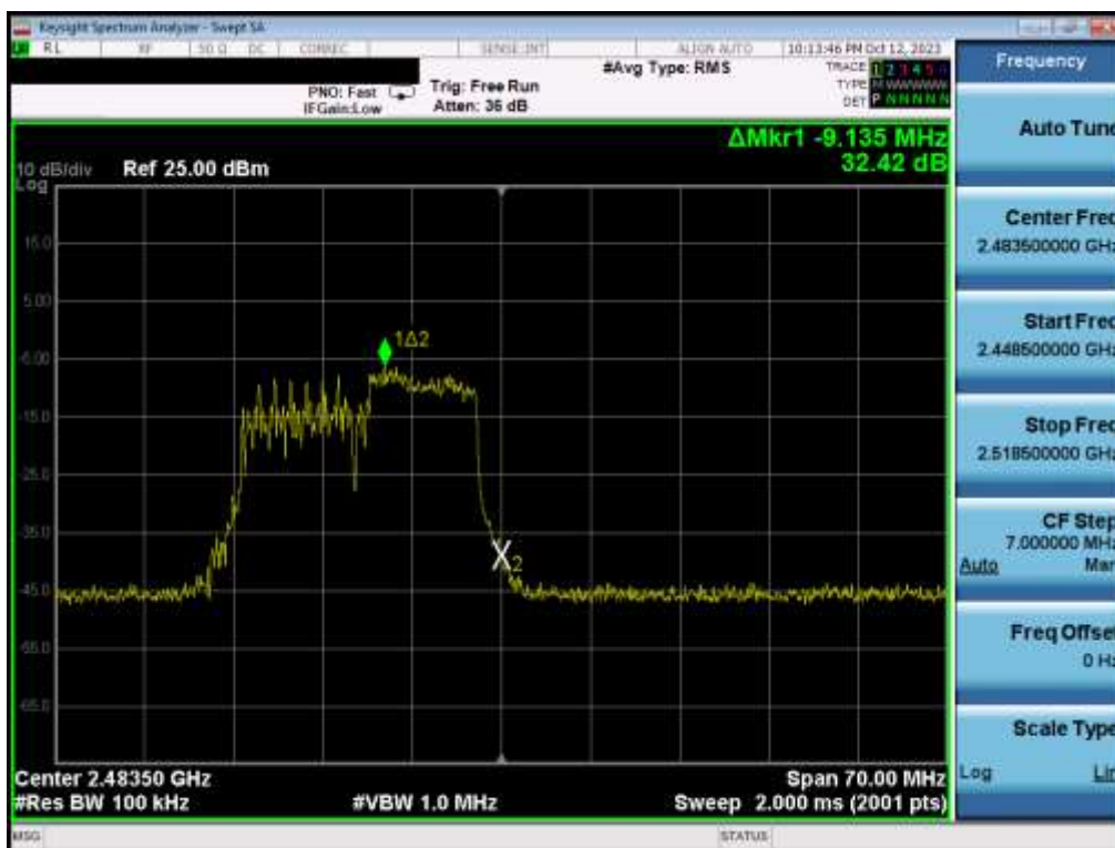
Plot 7-35. Band Edge Plot MIMO ANT1 (802.11be OFDMA – 106 Tones – Ch. 13)
