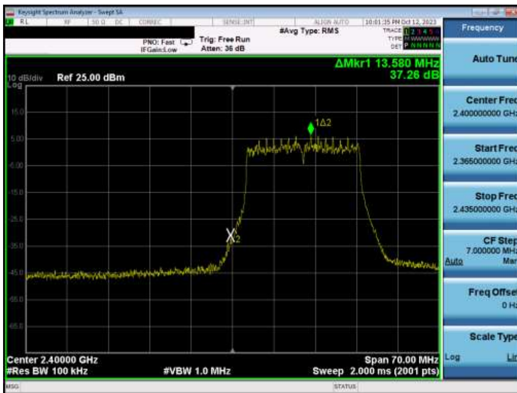
Plot 7-37. Band Edge Plot MIMO ANT1 (802.11be OFDMA – 242 Tones – Ch. 1)
