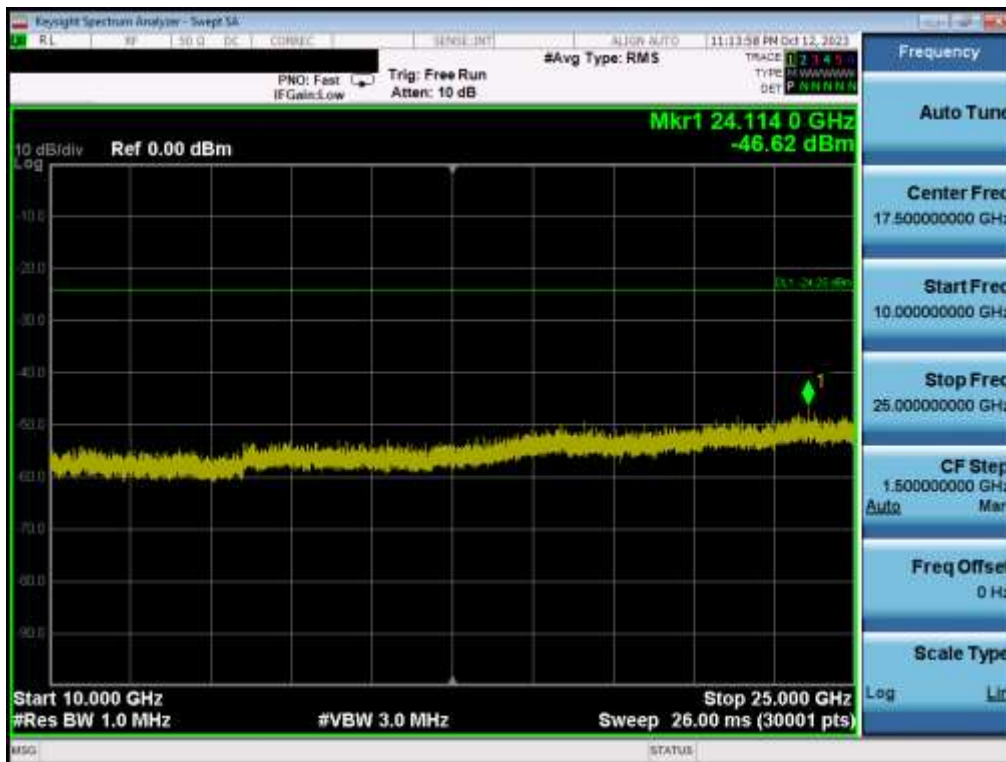
Plot 7-76. Conducted Spurious Plot MIMO ANT2 (802.11be OFDMA – 242 Tones – Ch. 11)
