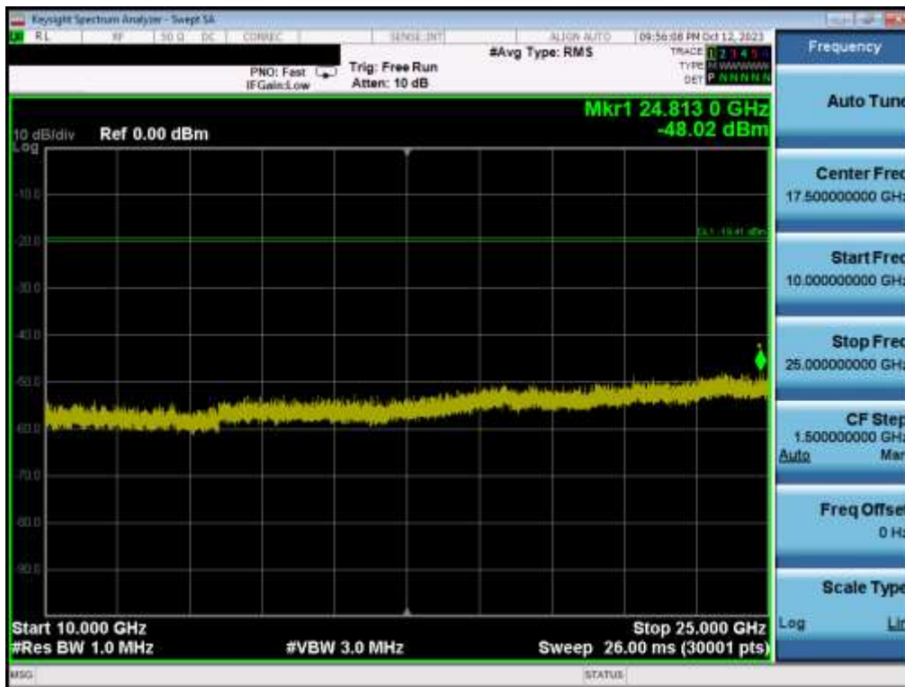
Plot 7-58. Conducted Spurious Plot MIMO ANT1 (802.11be OFDMA – 26 Tones – Ch. 11)
