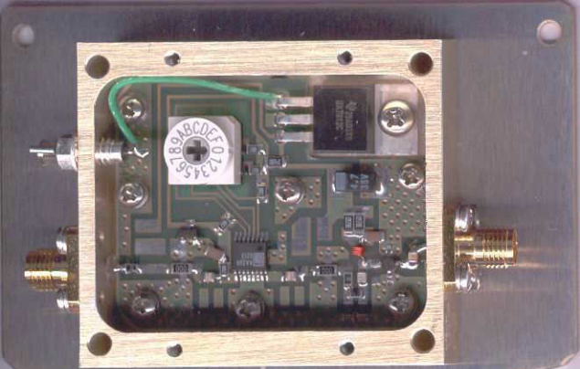
Uplink PreAmp of the IBDB-SMF
