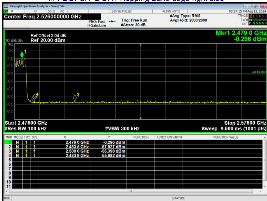
\pi/4 -DQPSK -2-DH1 Hopping Band edge-right side
