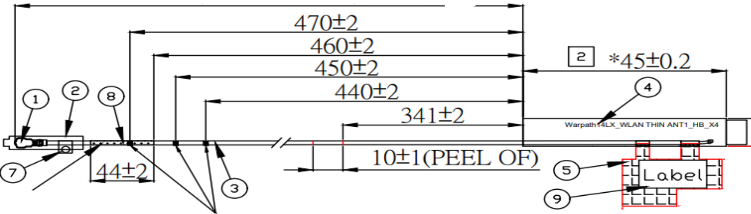
Tx1 (AUX) Antenna Dimensioned Drawing:
