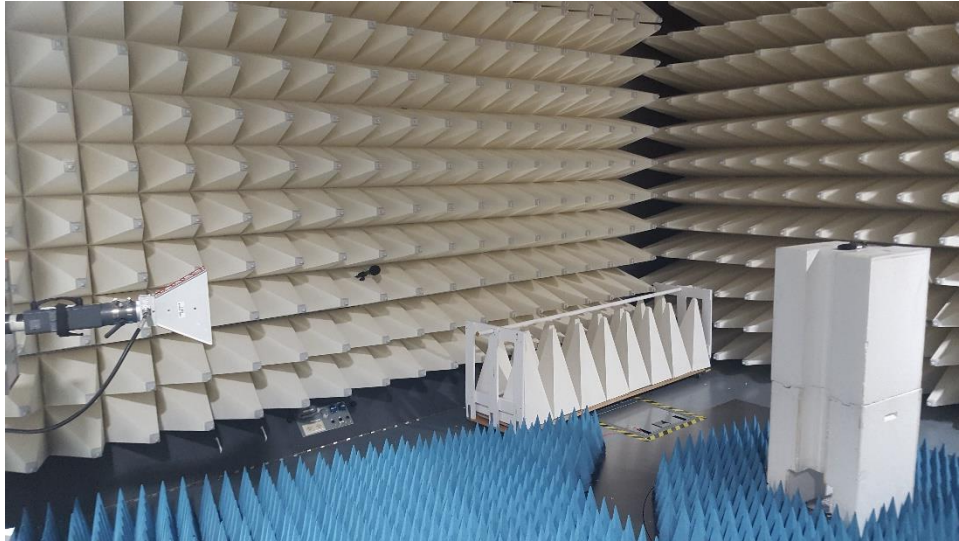
Figure B7. Radiated emission Test setup High Range
