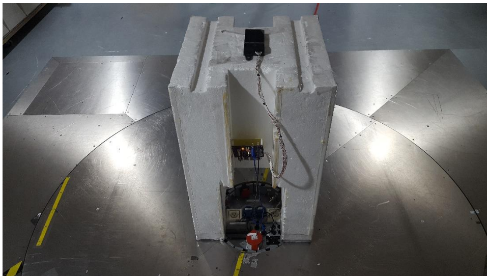
Figure B6. Radiated emission Test Setup Low Range – Back side
