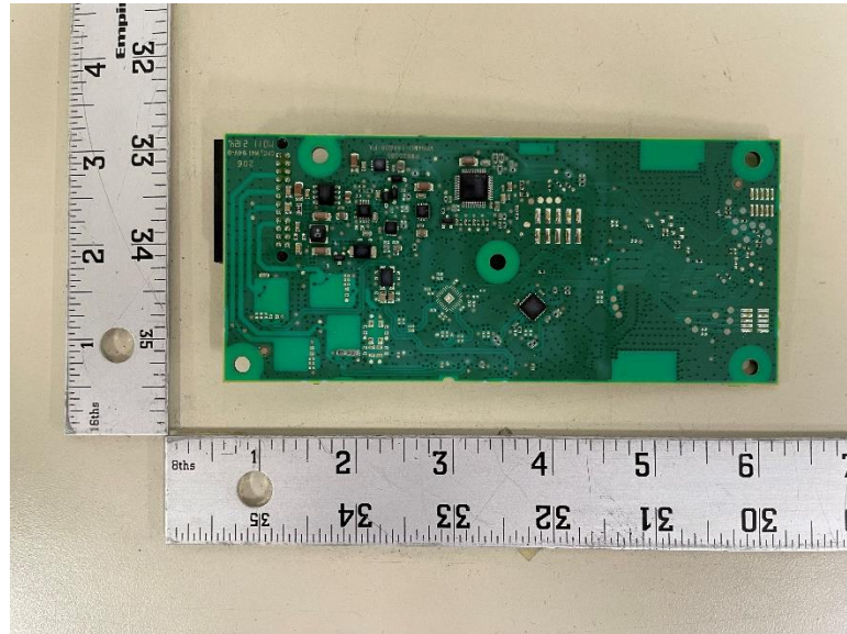
Figure B13. Radiated sample internal rear view
