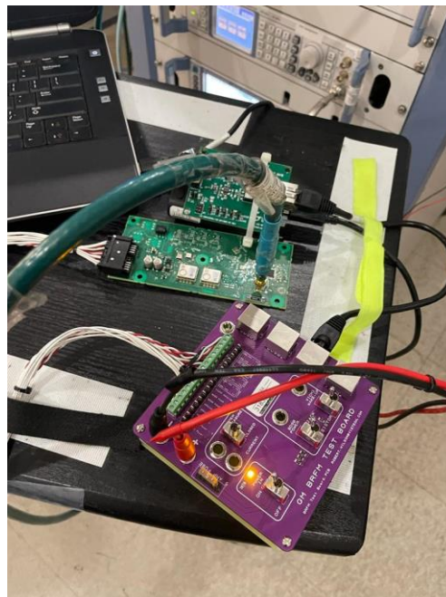
Figure B4. Conducted test setup
