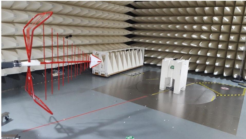
Figure B5. Radiated emission Test Setup Low Range
