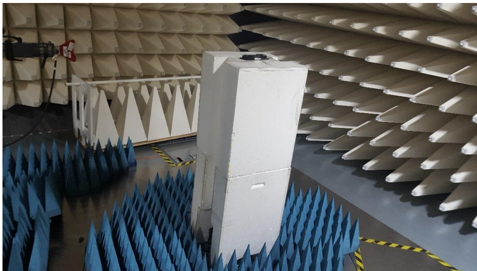
Figure B9. Radiated emission Test Setup High Range (>18GHz)
