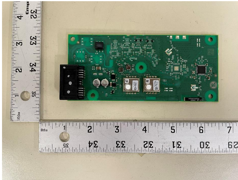
Figure B12. Radiated sample internal top view
