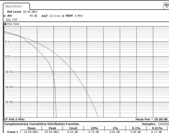
Band26-5MHz-16QAM-27015-1RB#0
