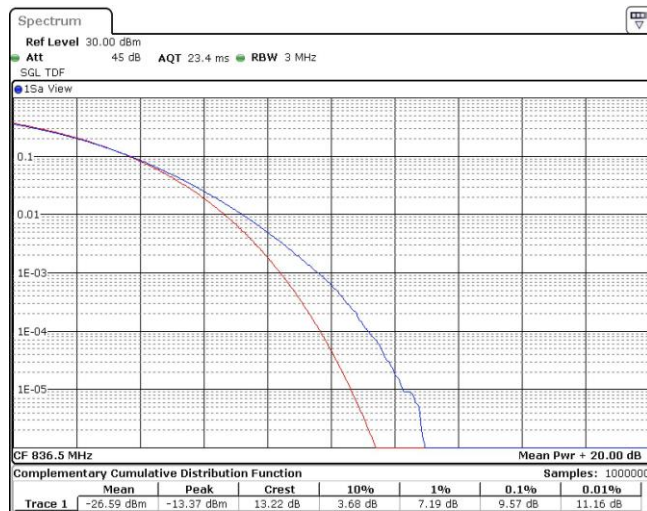
Band26-15MHz-QPSK-26915-75RB#0
