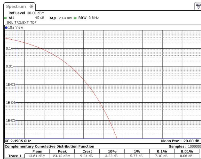
Band41-5MHz-QPSK-39675-25RB#0
