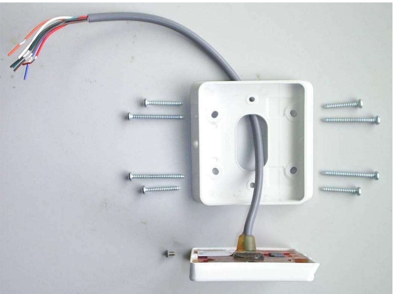
T12 Mifare - Assembly
