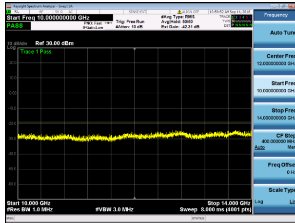
LTE20 Top+NB IoT GB (Upper) 10000MHz-14000MHz
