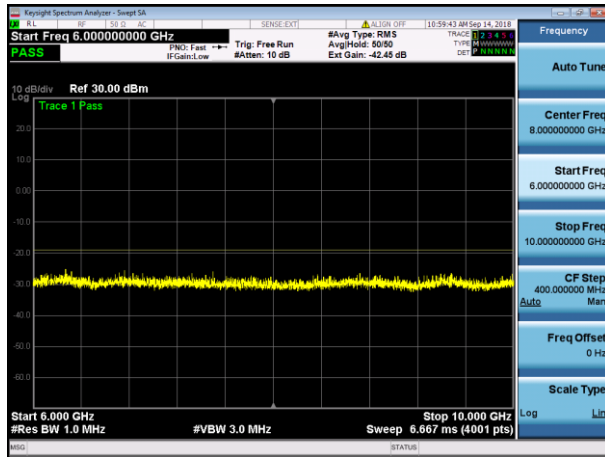
LTE20 Top+NB IoT GB (Upper) 6000MHz-10000MHz
