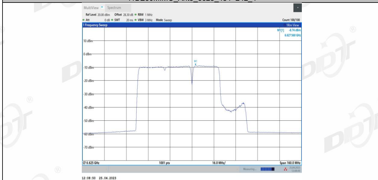
11BE80MIMO Ant4 6625 484+242_1
