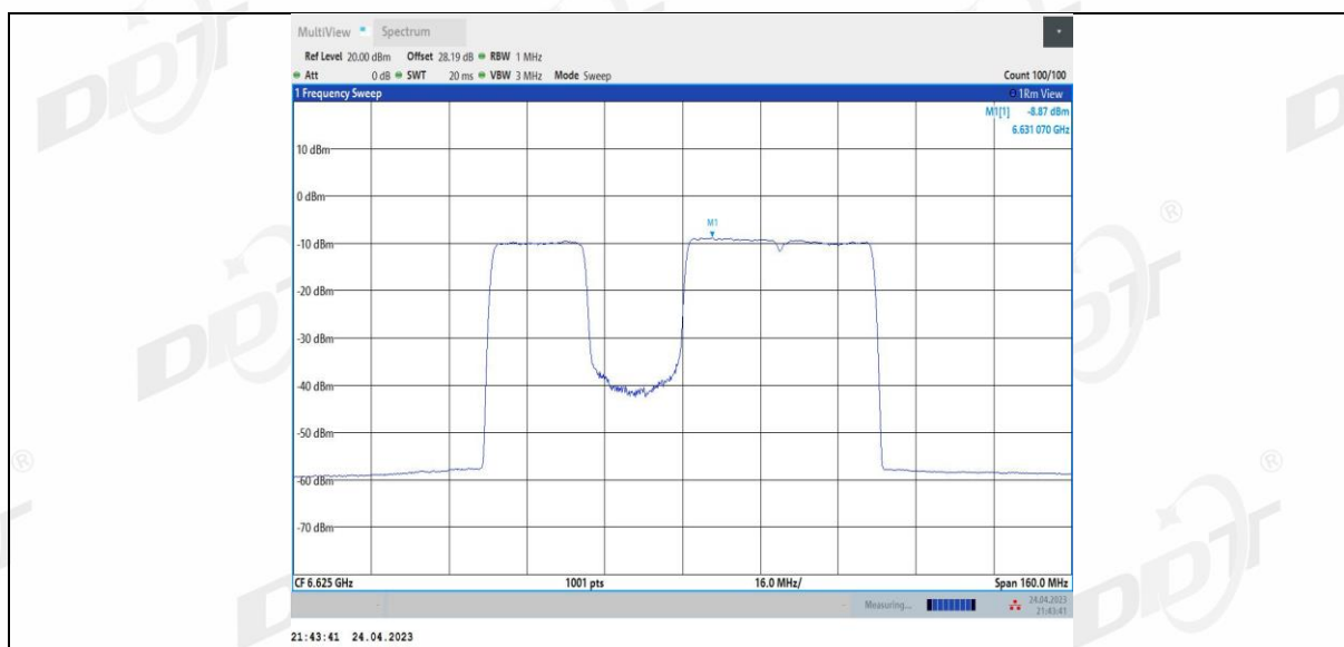
11BE80MIMO Ant3 6625 484+242_3
