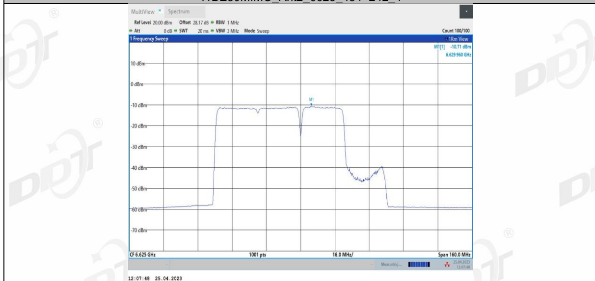
11BE80MIMO Ant3 6625 484+242 1
