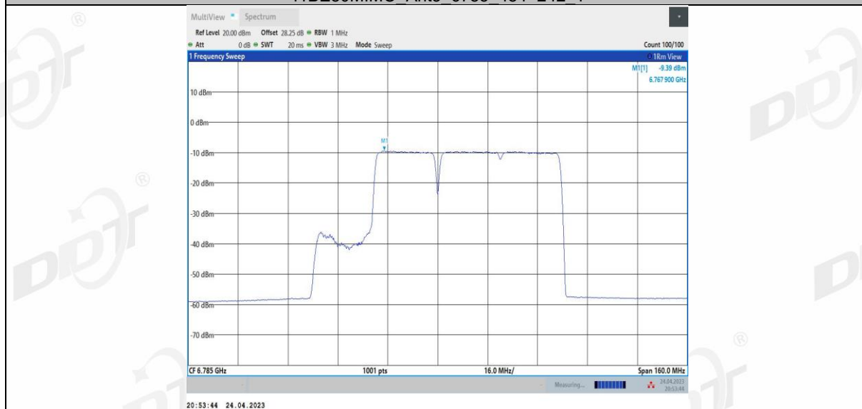
11BE80MIMO Ant3 6785 484+242 2
