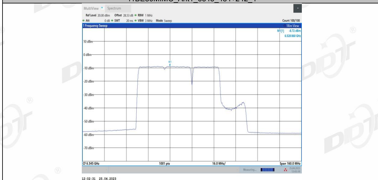
11BE80MIMO Ant2 6545 484+242 1
