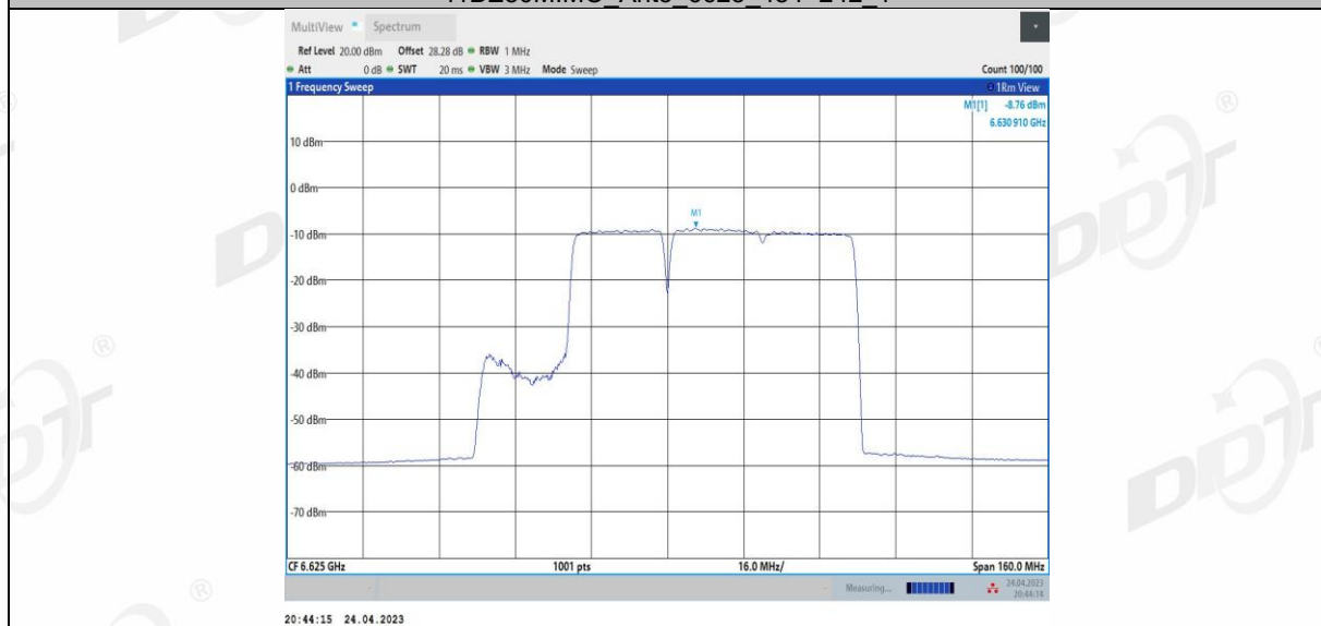
11BE80MIMO Ant3 6625 484+242 2
