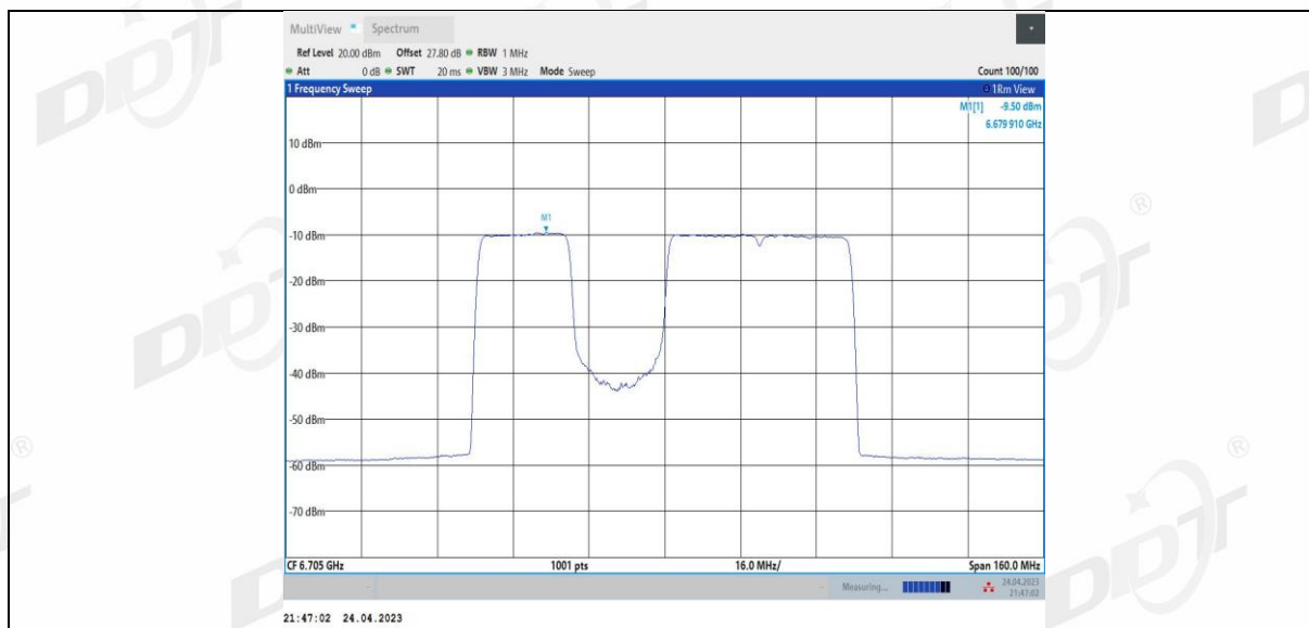
11BE80MIMO Ant2 6705 484+242_3
