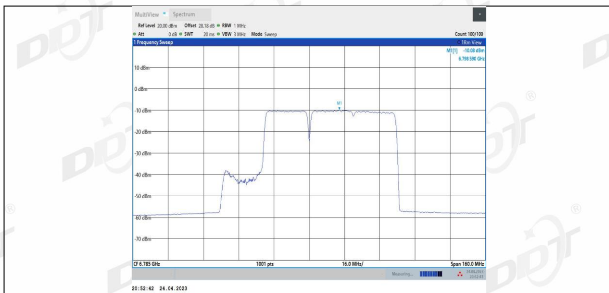
11BE80MIMO Ant2 6785 484+242 2
