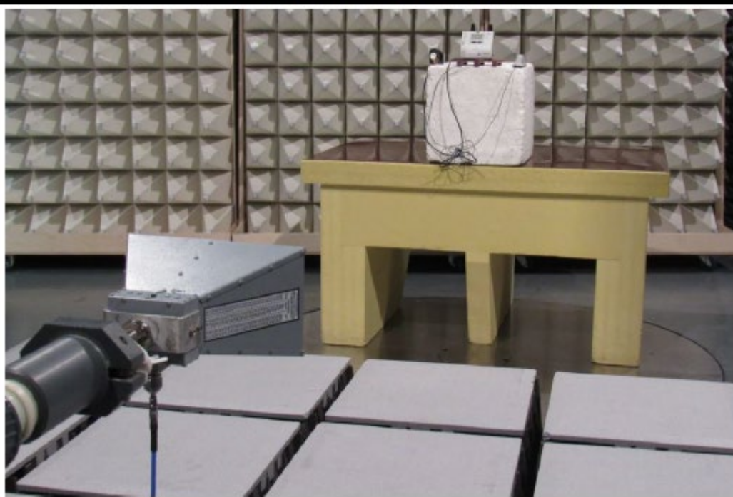
TEST SETUP 1GHz - 10GHz
