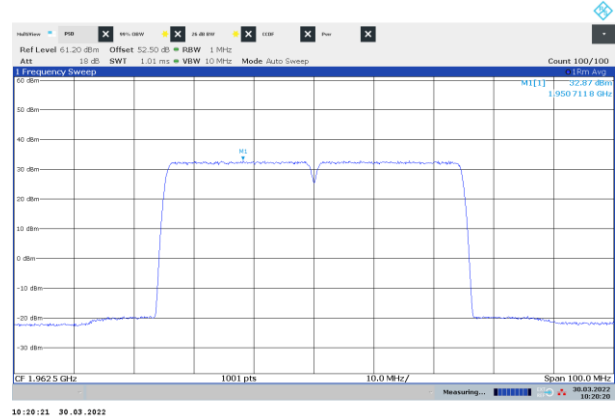
Figure 8.2-10: PSD of NR 25 MHz channel bandwidth, two-carrier operation, sample plot, middle channels
