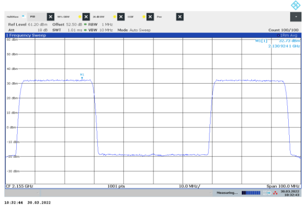
Figure 8.1-10: PSD of NR 25 MHz channel bandwidth, two-carrier operation, sample plot, bottom and top channels
