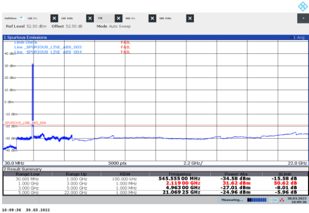
Figure 8.3-25: Conducted spurious emissions of multi-RAT operation, LTE 20 MHz + 2 * NR 25 MHz, bottom
