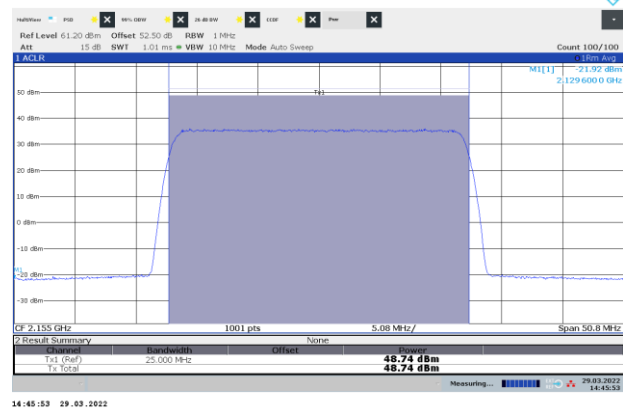
Figure 8.1-14: Power of NR 25 MHz channel bandwidth, single carrier operation, sample plot, mid channel
