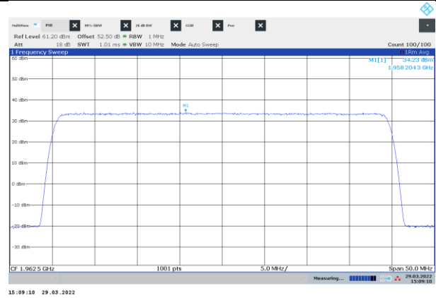
Figure 8.2-8: PSD of NR 40 MHz channel bandwidth, single carrier operation, sample plot, mid channel
