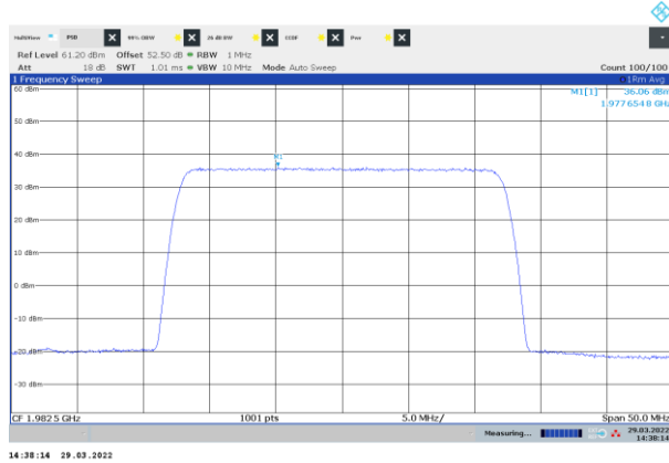
Figure 8.2-3: PSD of NR 25 MHz channel bandwidth, single carrier operation, sample plot, top channel
