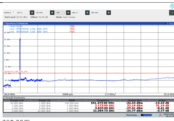
Figure 8.3-18: Conducted spurious emissions of NR 25 MHz three-carrier operation, top
