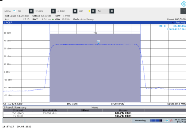
Figure 8.2-13: Power of NR 25 MHz channel bandwidth, single carrier operation, sample plot, bottom channel
