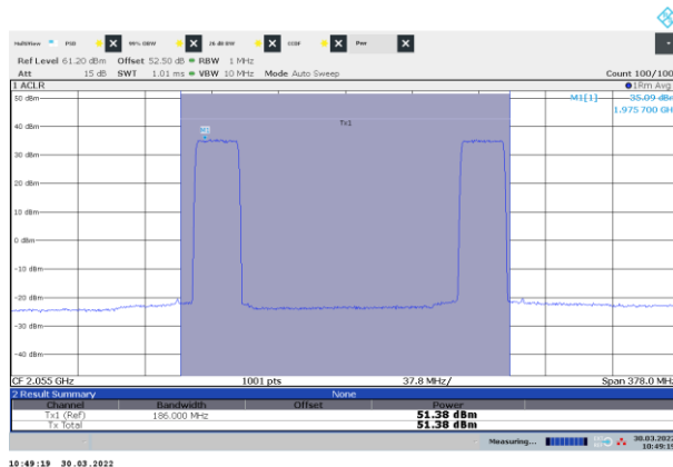
Figure 8.2-24: Power of NR 25 MHz channel bandwidth, two-carrier operation (1x 25 MHz band 25 + 1x 25 MHz band 66), sample plot, top channel band 25 and bottom channel band 66
