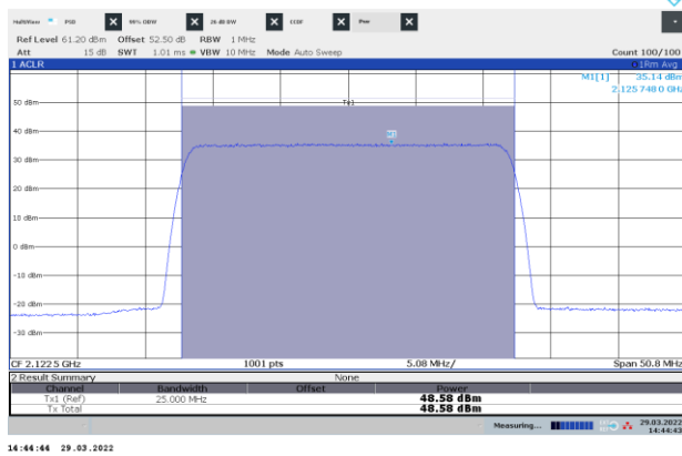
Figure 8.1-13: Power of NR 25 MHz channel bandwidth, single carrier operation, sample plot, bottom channel
