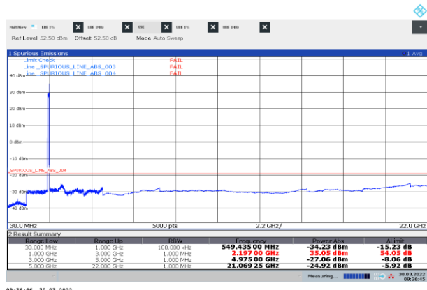
Figure 8.3-21: Conducted spurious emissions of NR 40 MHz three-carrier operation 2 x NR 40 MHz+ 1 x NR 5 MHz, bottom
