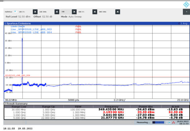
Figure 8.3-12: Conducted spurious emissions of NR 25 MHz two-carrier operation, top
