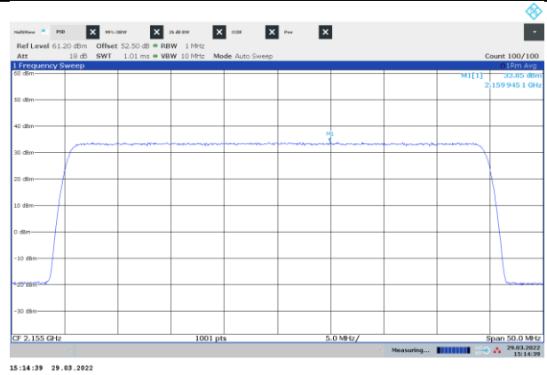
Figure 8.1-8: PSD of NR 40 MHz channel bandwidth, single carrier operation, sample plot, mid channel
