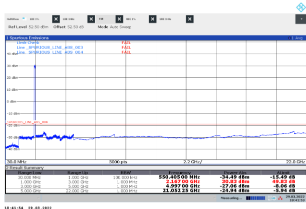
Figure 8.3-19: Conducted spurious emissions of NR 30 MHz three-carrier operation, bottom
