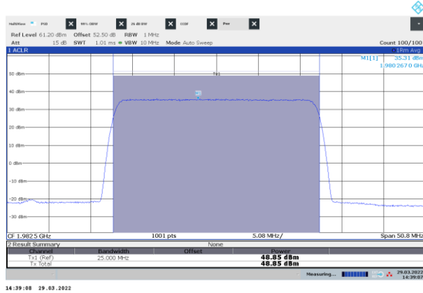
Figure 8.2-15: Power of NR 25 MHz channel bandwidth, single carrier operation, sample plot, top channel
