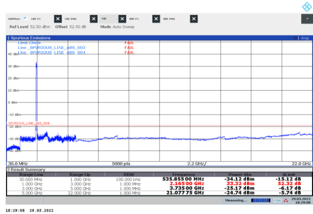
Figure 8.3-14: Conducted spurious emissions of NR 30 MHz two-carrier operation, top
