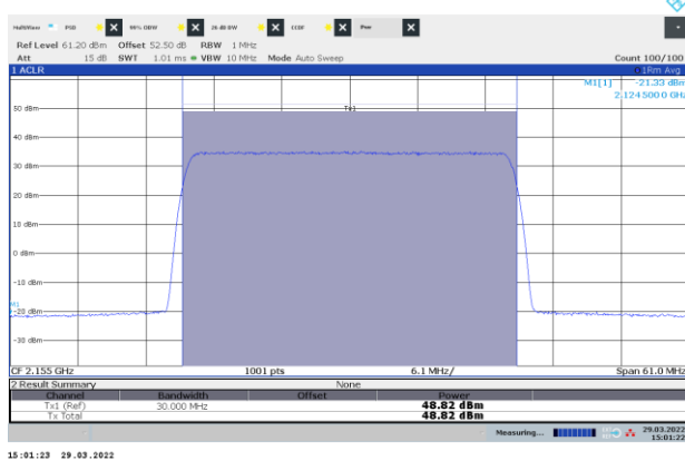
Figure 8.1-17: Power of NR 30 MHz channel bandwidth, single carrier operation, sample plot, mid channel
