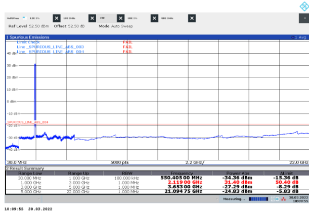
Figure 8.3-26: Conducted spurious emissions of multi-RAT operation, LTE 20 MHz + 2 * NR 25 MHz, top
