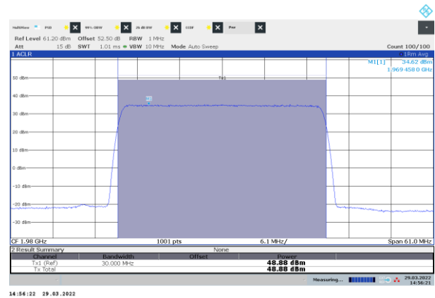
Figure 8.2-18: Power of NR 30 MHz channel bandwidth, single carrier operation, sample plot, top channel
