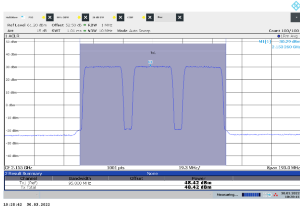
Figure 8.1-23: Power of NR 25 MHz channel bandwidth, three-carrier operation, sample plot, mid channel
