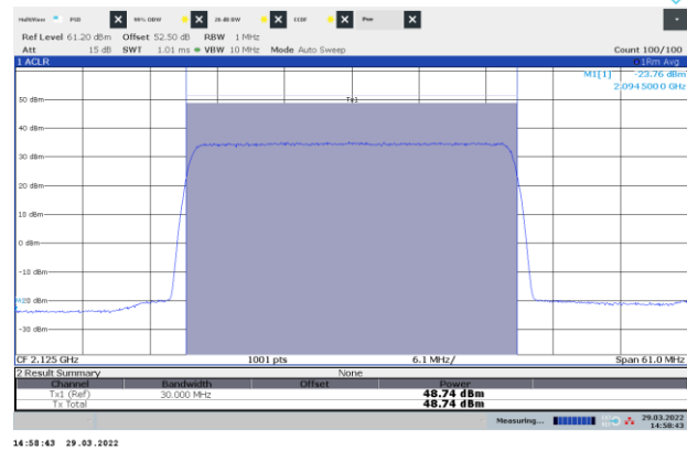
Figure 8.1-16: Power of NR 30 MHz channel bandwidth, single carrier operation, sample plot, bottom channel
