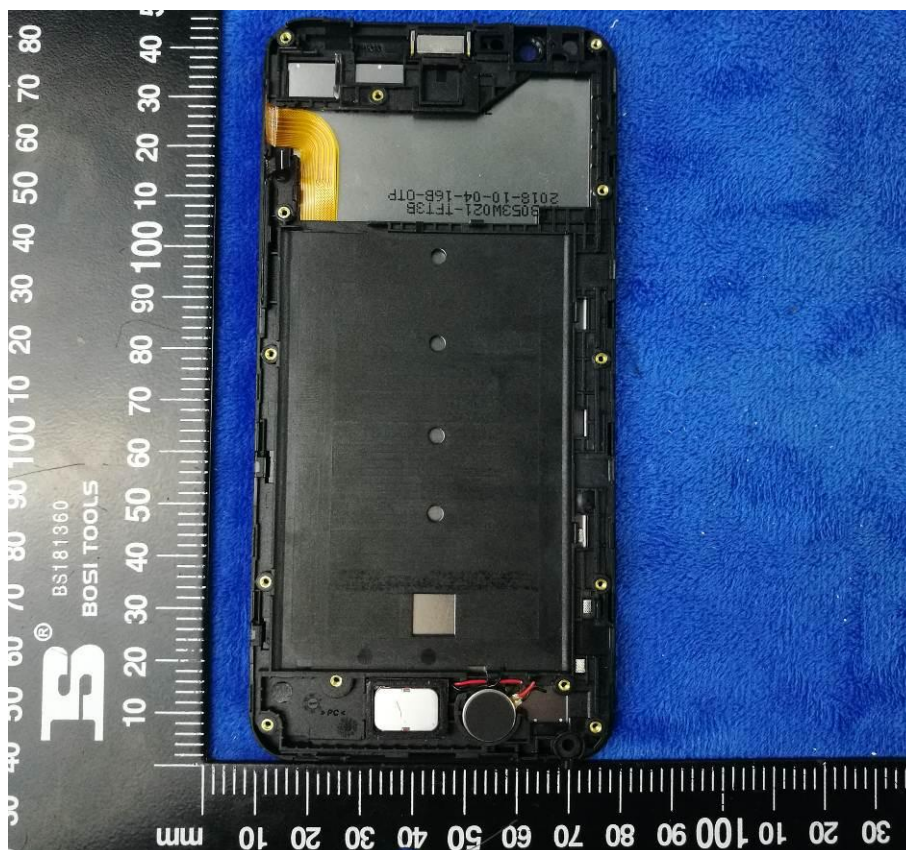
LCD- Rear View
