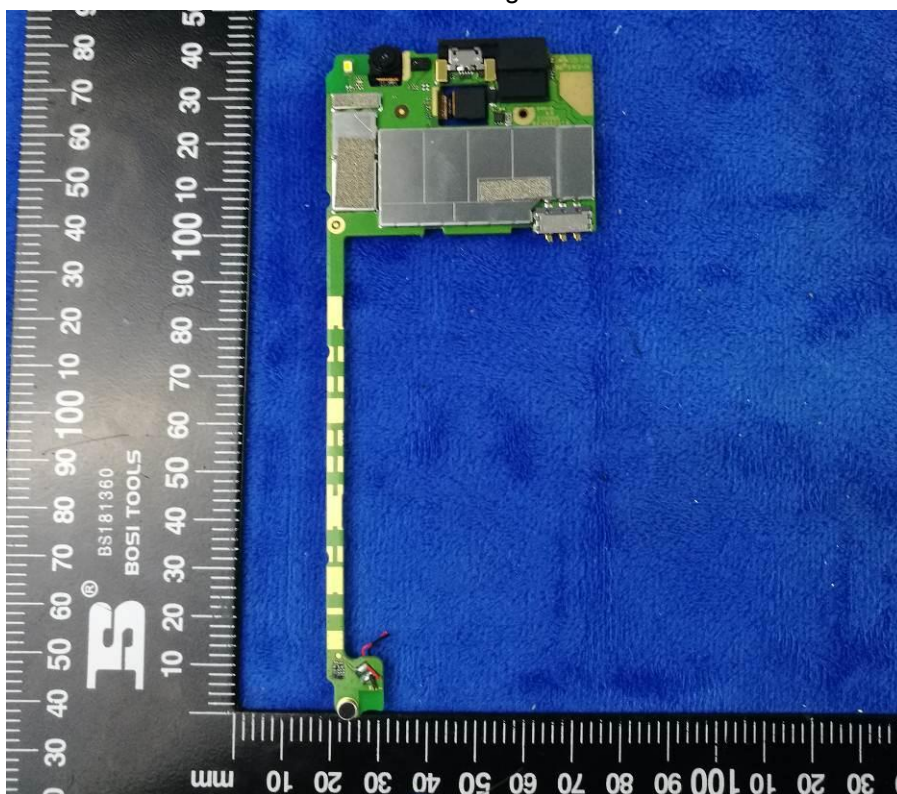
Mainboard with Shielding – Front View
