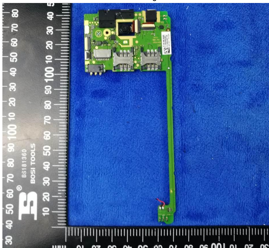
Mainboard with Shielding – Rear View
