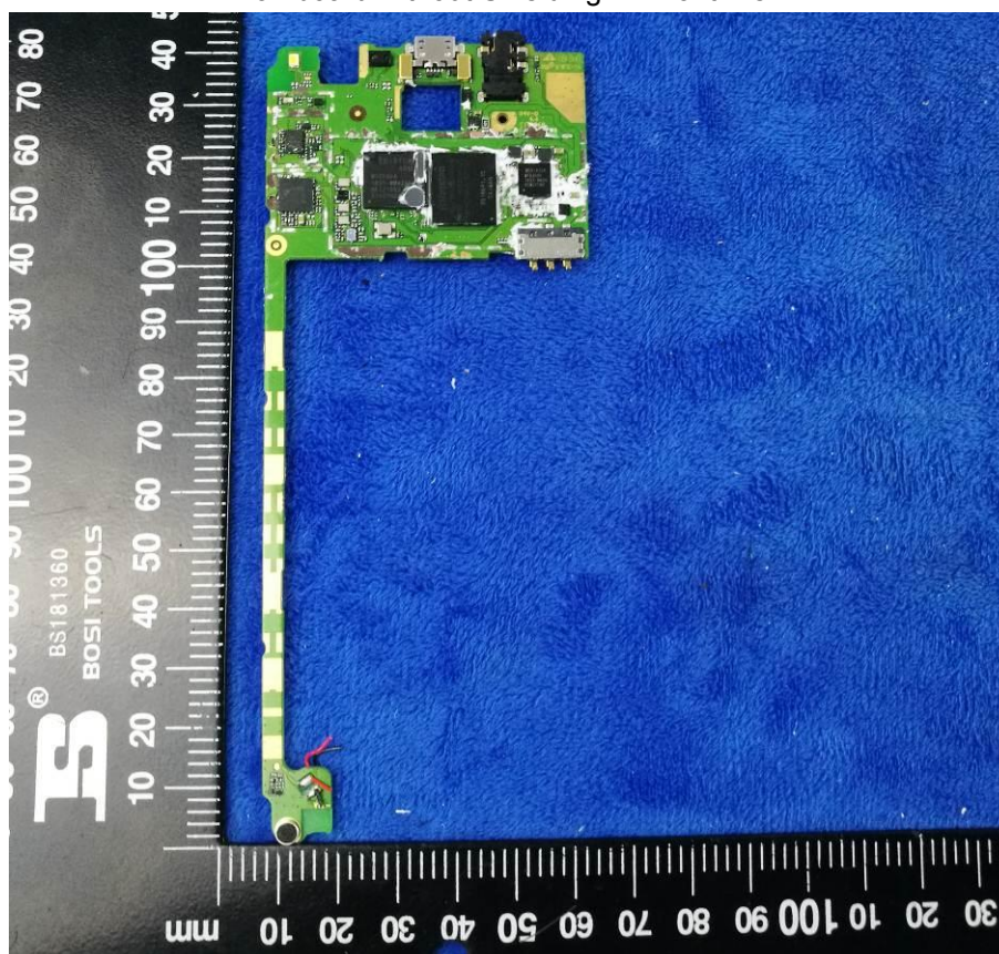
Mainboard without Shielding – Front View
