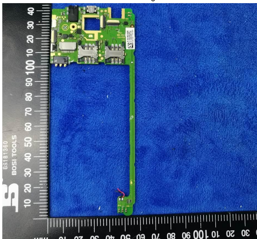
Mainboard without Shielding – Rear View
