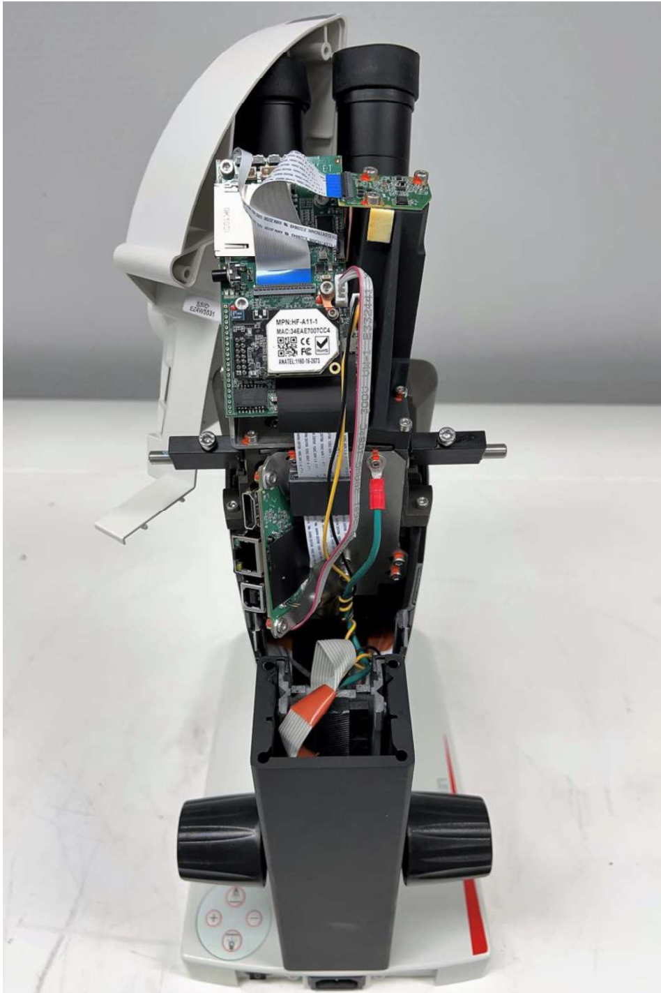
EZ4 W: rear view inside, assembling and connections
