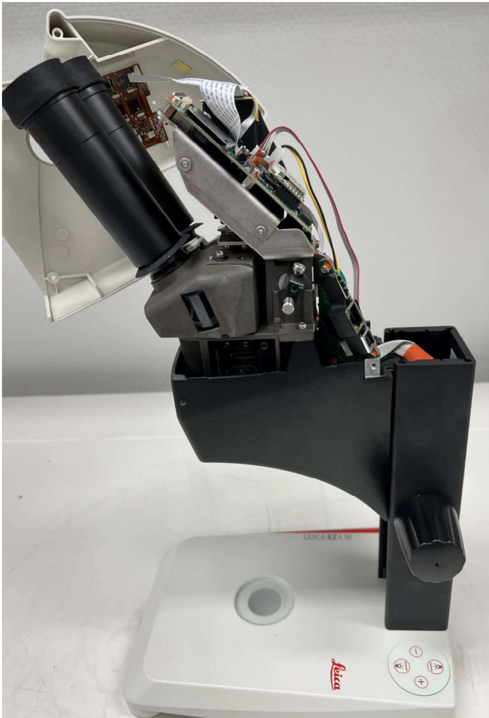
Figure 6 EZ4 W: left view inside
