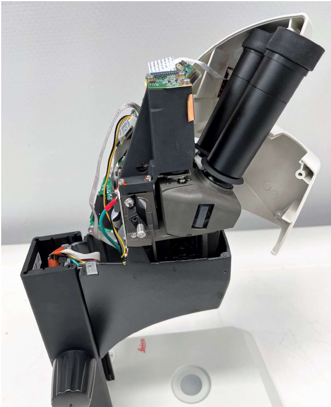
EZ4 W: rightt view inside
