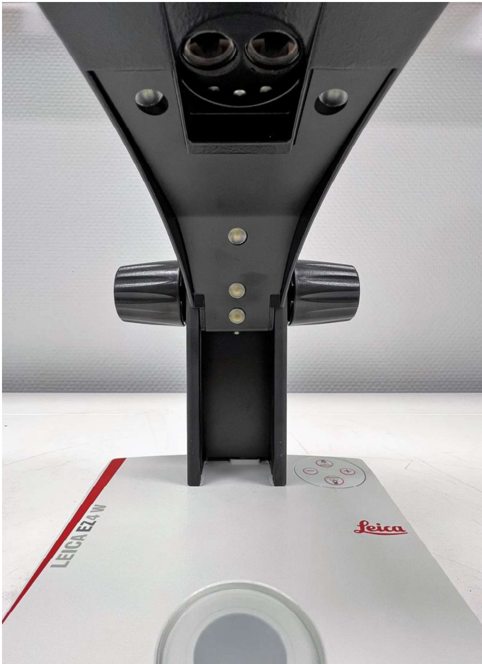
EZ4 W: Front view Illumination parts and LED's
