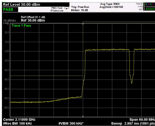
Low Band Edge, 2 Carrier, Modulation: 64QAM, BW=20MHz
