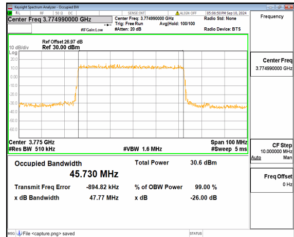
n78(3700-3800MHz) 50M DFT-s-OFDM 64QAM Outer_Full High
