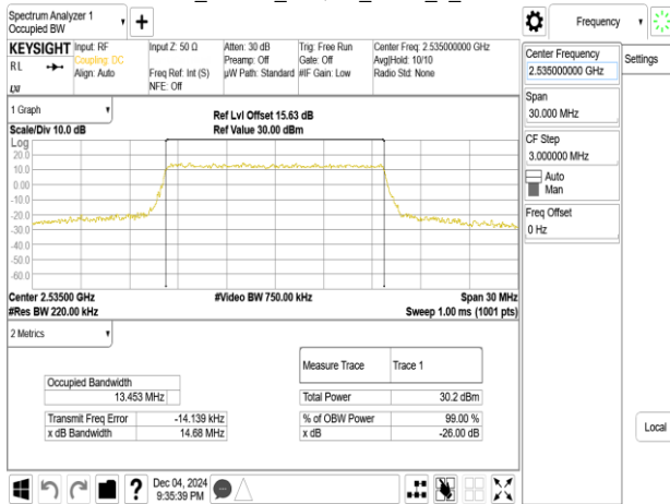
Band7_15MHz_256QAM_RB75_0_CH21100
