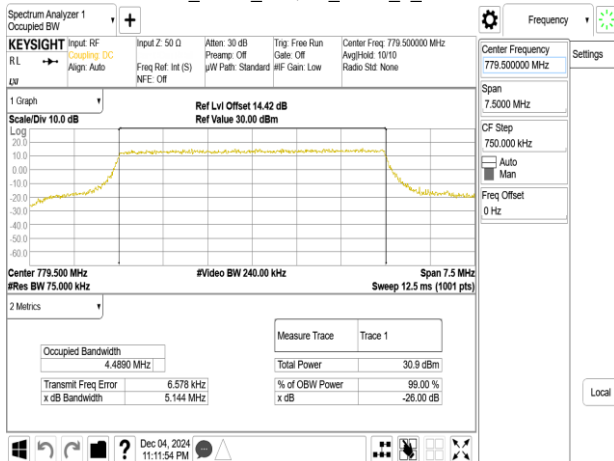
Band13_5MHz_64QAM_RB25_0_CH23205
