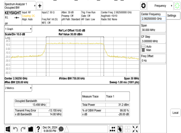
Band7_15MHz_64QAM_RB75_0_CH21375
