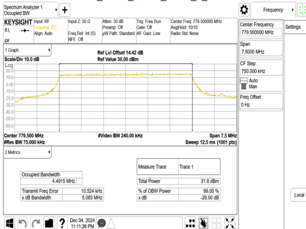
Band13_5MHz_16QAM_RB25_0_CH23205
