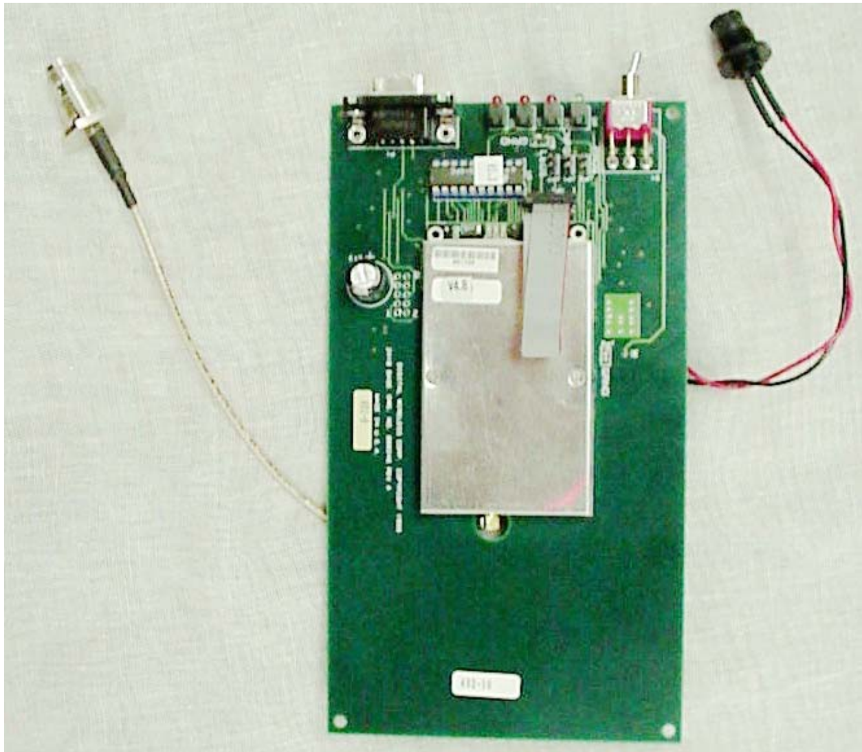
Photo 4. EUT, Top View of PCB
