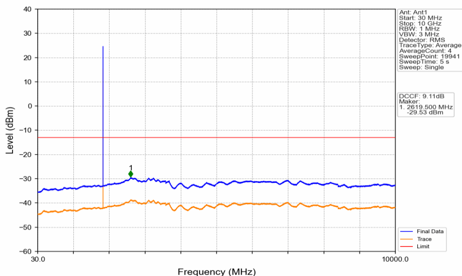
PCS1900_GPRS_LCH_1850.2MHz_1 TX Slot_NTNV
