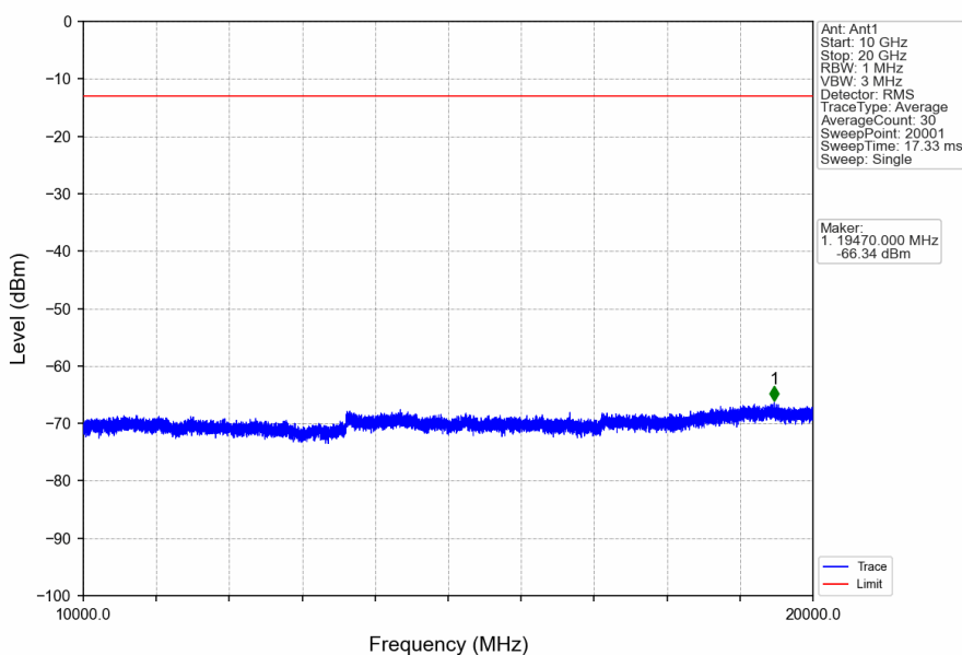
Band2_RMC_LCH_1852.4MHz_12.2kbps RMC_NTNV
