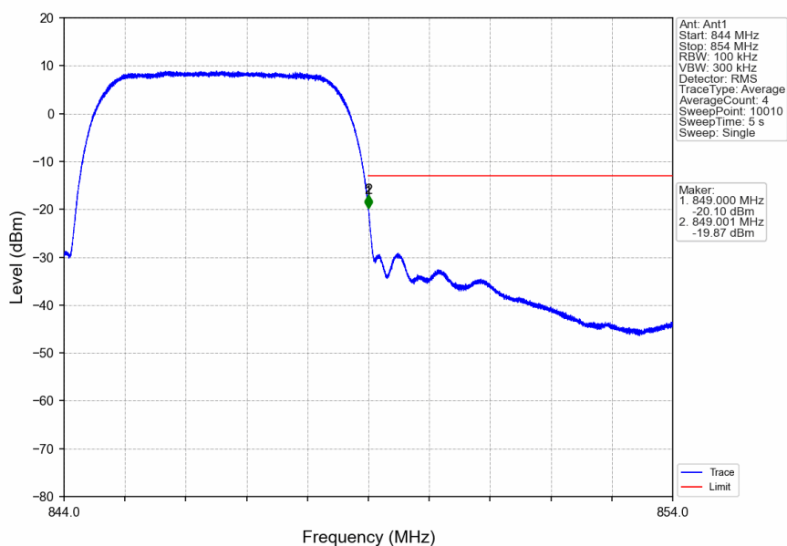
Band5_RMC_HCH_846.6MHz_12.2kbps RMC_NTNV
