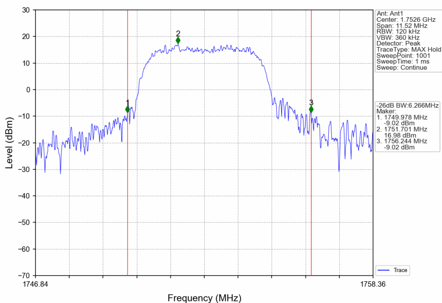
Band4_HSUPA_HCH_1752.6MHz_Subtest 1_NTNV
