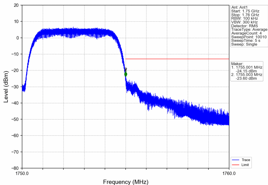
Band4_HSUPA_HCH_1752.6MHz_Subtest 1_NTNV
