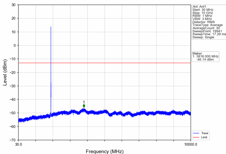
Band2_HSDPA_HCH_1907.6MHz_Subtest 1_NTNV
