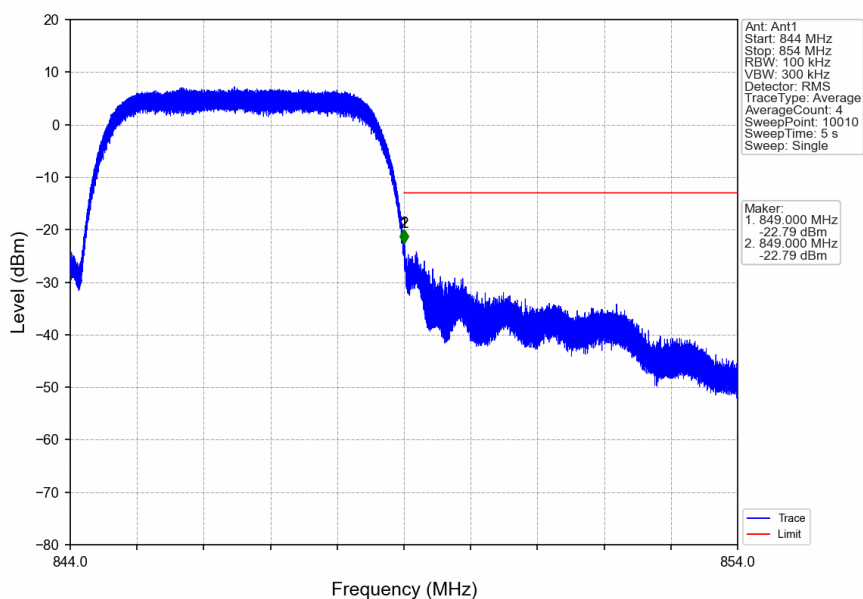
Band5_HSDPA_HCH_846.6MHz_Subtest 1_NTNV
