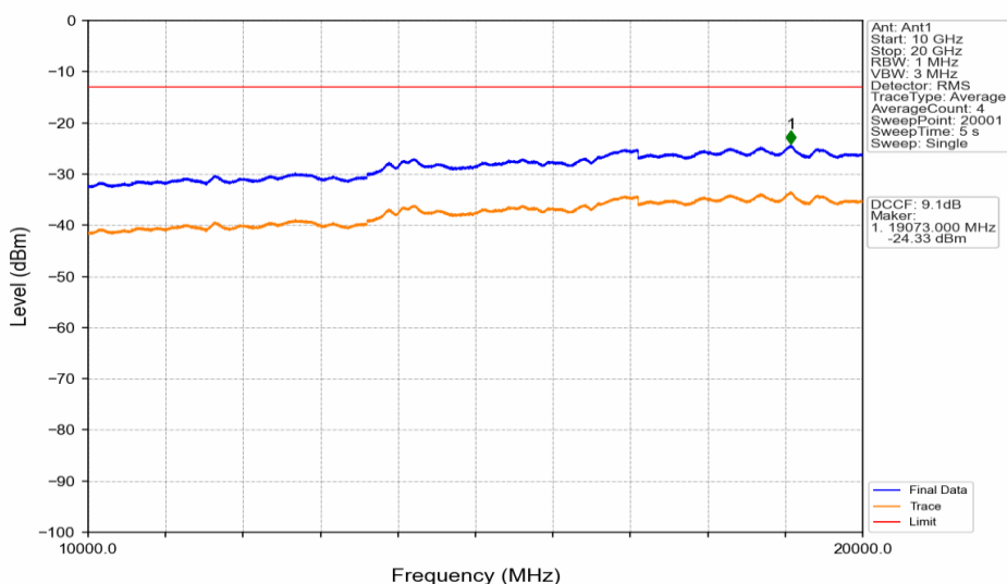
PCS1900_GPRS_MCH_1880MHz_1 TX Slot_NTNV
