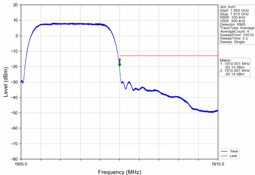
Band2_RMC_HCH_1907.6MHz_12.2kbps RMC_NTNV
