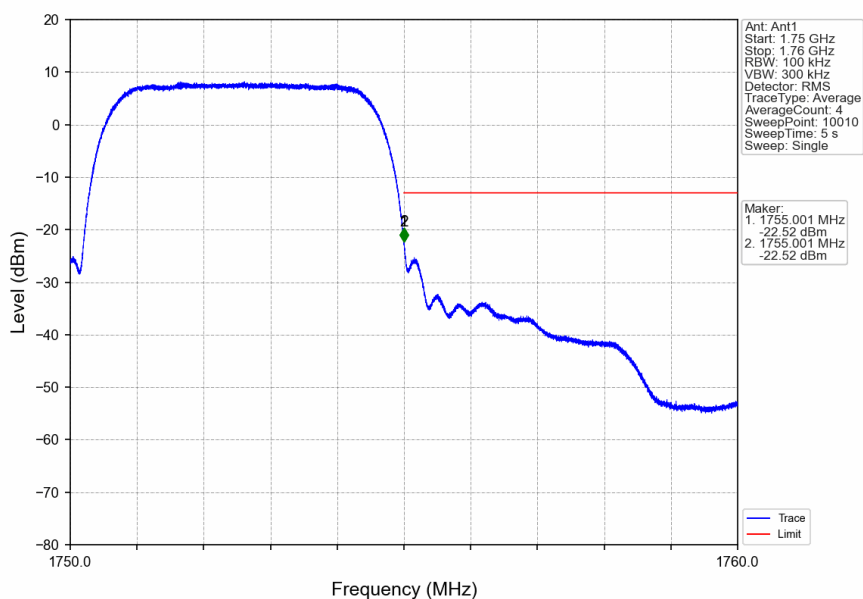
Band4_RMC_HCH_1752.6MHz_12.2kbps RMC_NTNV
