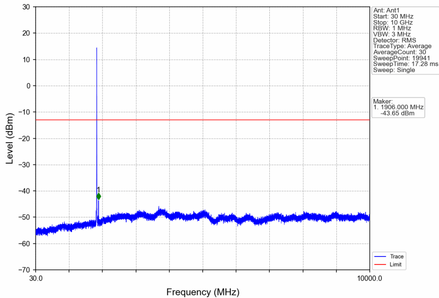
Band2_HSUPA_LCH_1852.4MHz_Subtest 1_NTNV
