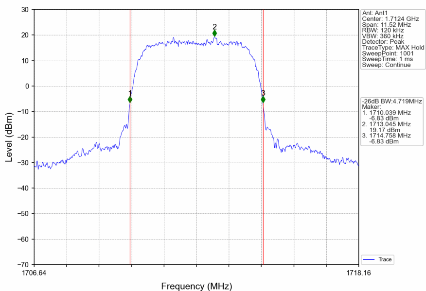
Band4_RMC_LCH_1712.4MHz_12.2kbps RMC_NTNV
