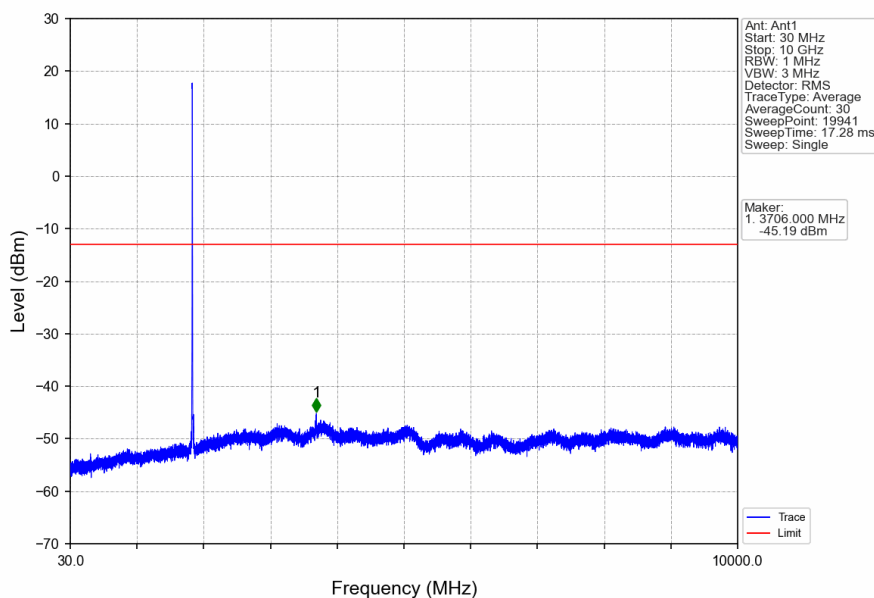
Band2_RMC_LCH_1852.4MHz_12.2kbps RMC_NTNV
