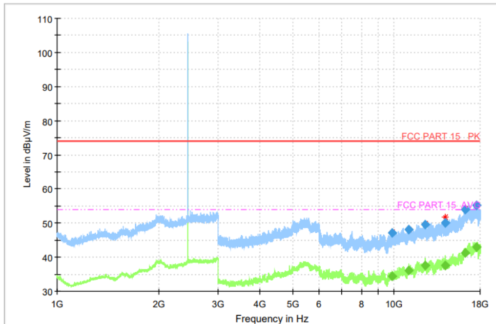
Fig. 39 Radiated Spurious Emission ( \pi/4 DQPSK, Ch39, 1GHz ~ 18GHz)
