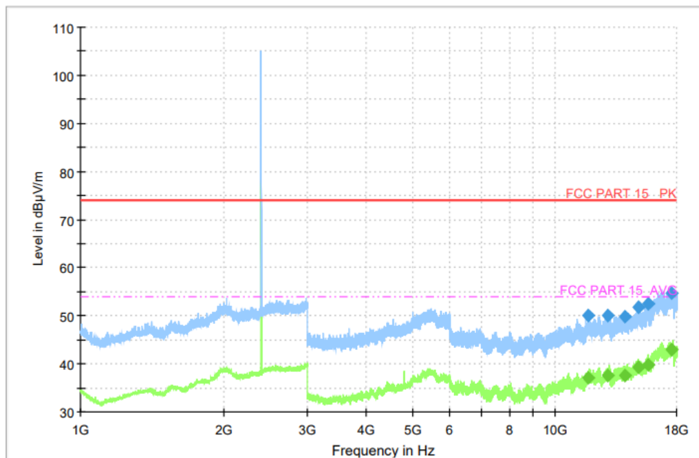
Fig. 43 Radiated Spurious Emission (8DPSK, Ch0, 1GHz ~ 18GHz)
