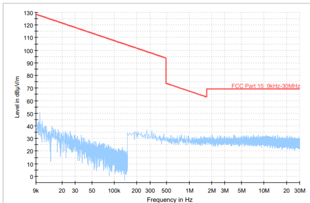
Fig. 48 Radiated Spurious Emission (All Channels, 9kHz ~ 30MHz)
