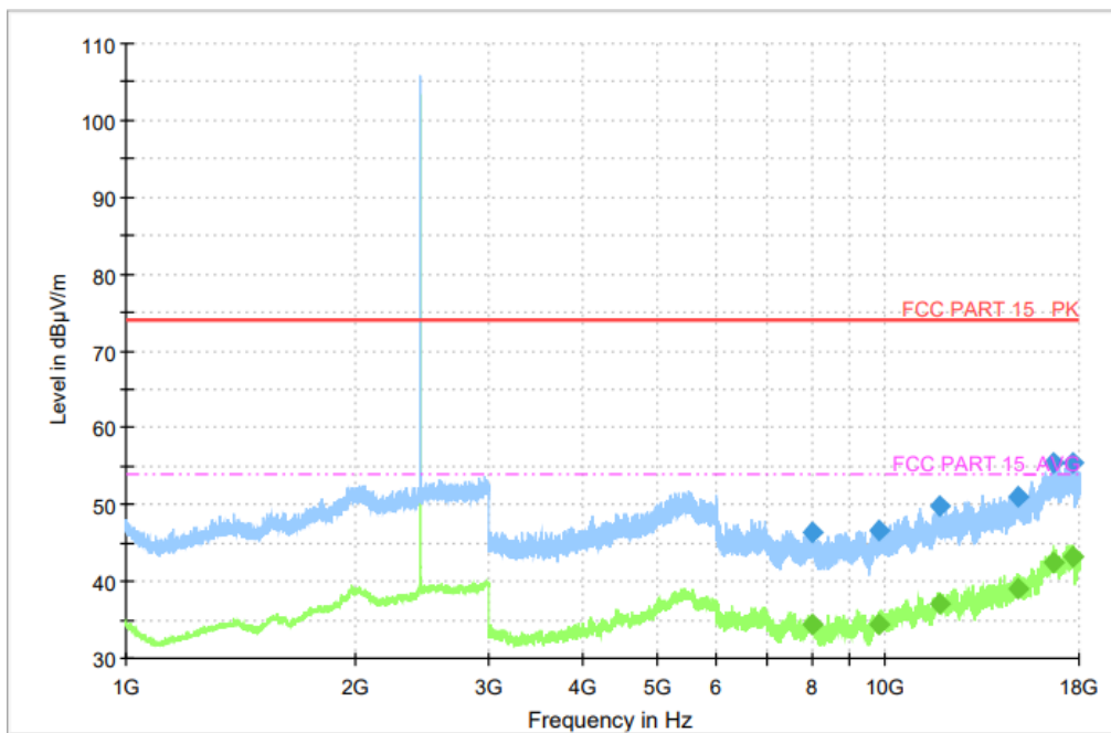
Fig. 34 Radiated Spurious Emission (GFSK, Ch39, 1GHz ~ 18GHz)
