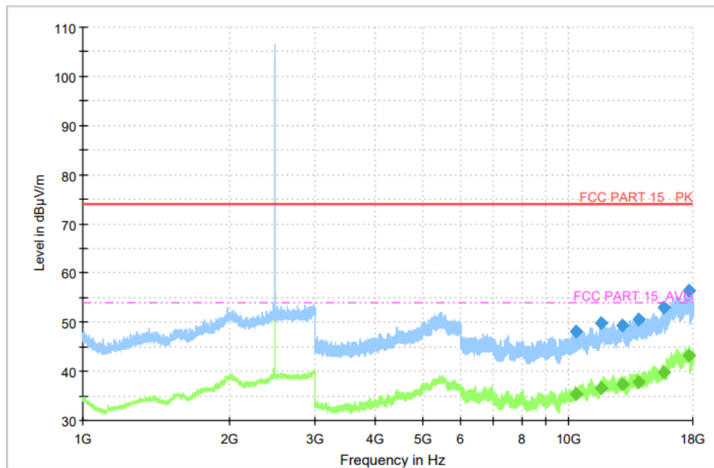
Fig. 35 Radiated Spurious Emission (GFSK, Ch78, 1GHz ~ 18GHz)
