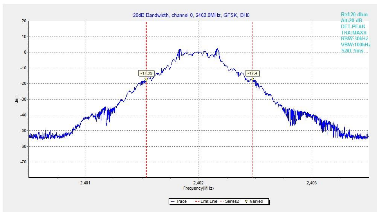
Fig. 51 20dB Bandwidth (GFSK, Ch 0)
