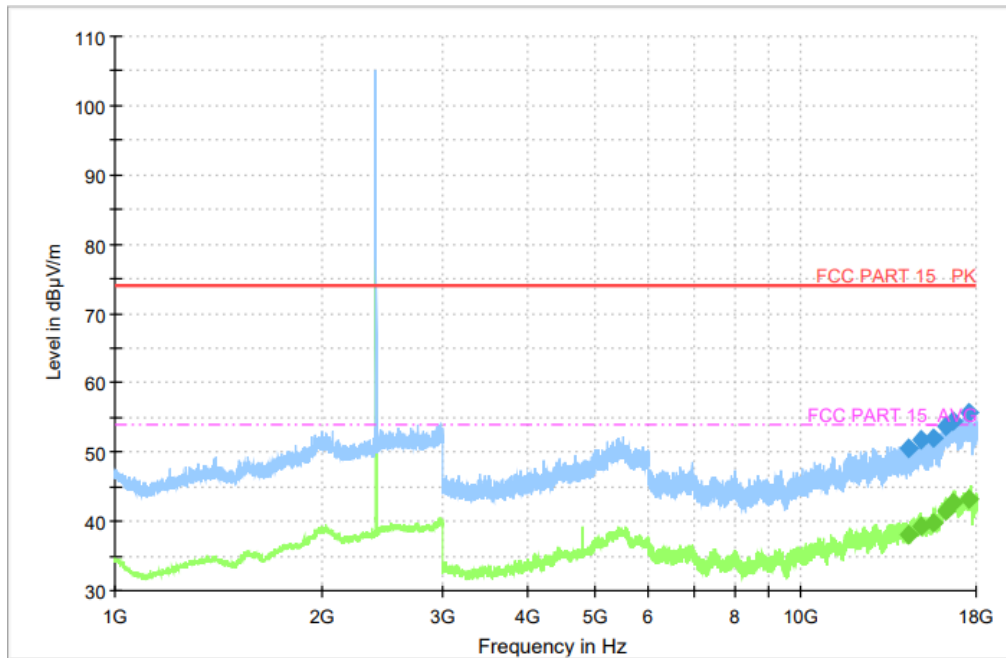
Fig. 33 Radiated Spurious Emission (GFSK, Ch0, 1GHz ~ 18GHz)
