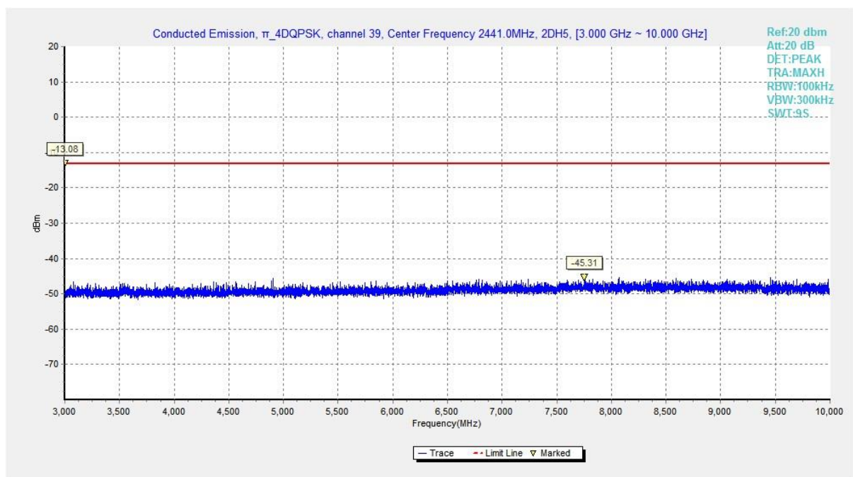
Fig. 22 Conducted Spurious Emission ( \pi/4 DQPSK, Ch39, 3GHz-10GHz)
