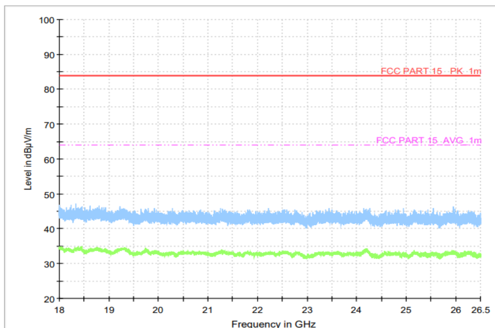
Fig. 50 Radiated Spurious Emission (All Channels, 18GHz ~ 26.5GHz)
