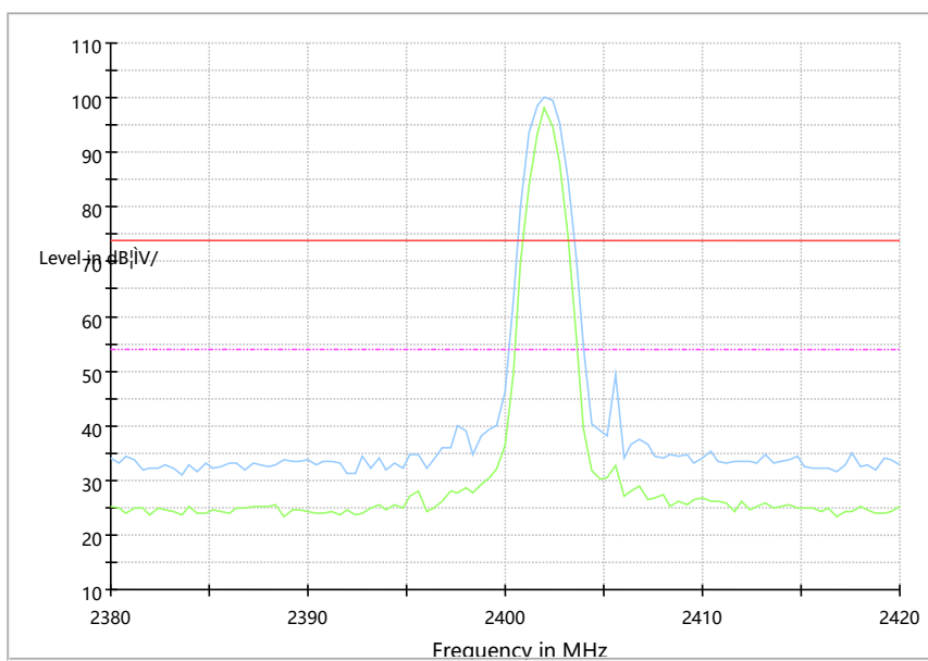
Radiated Emission Band Edge for 2402MHz
