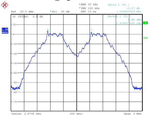
DH1_High 1.001MHz
