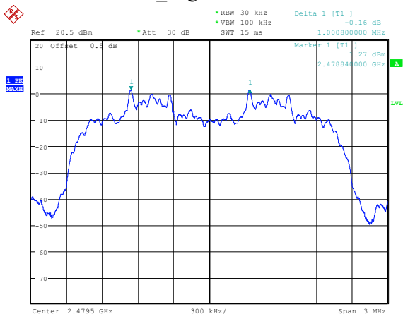
2DH1_High 1.001MHz
