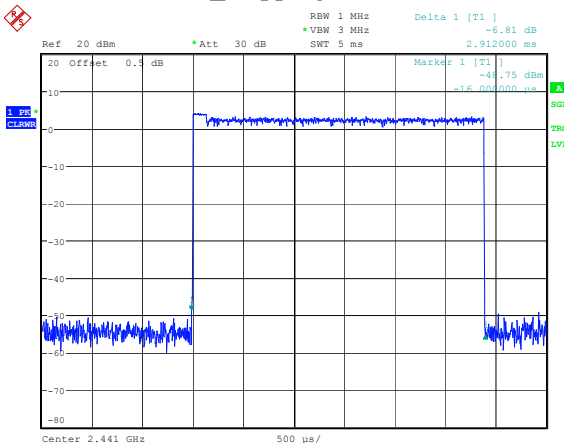
2DH5_Hopping 2.912ms
