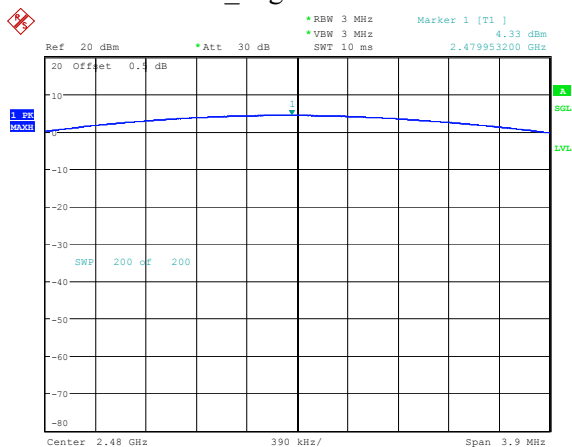
DH1_High 4.33dBm
