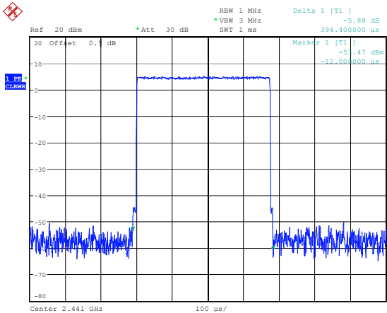
DH1_Hopping 0.394ms
