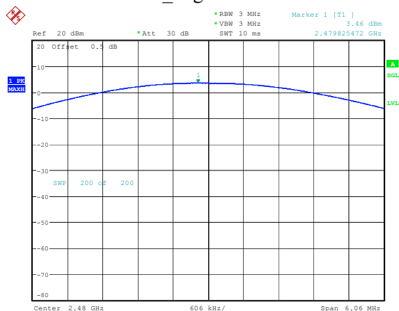
2DH1_High 3.46dBm
