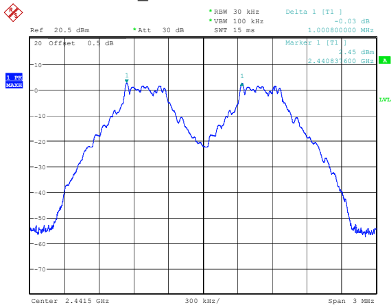
DH1_Middle 1.001MHz
