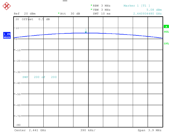
DH1_Middle 5.08dBm
