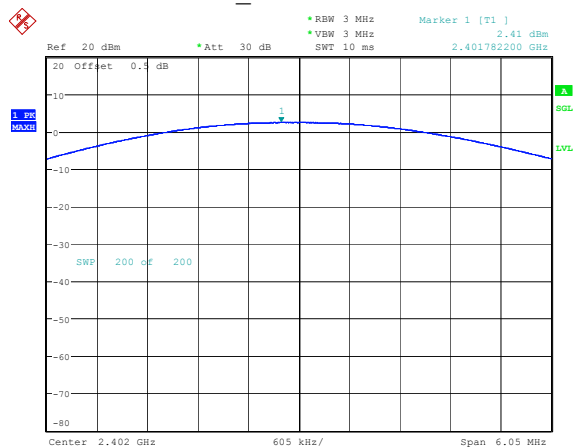
2DH1_Low 2.41dBm
