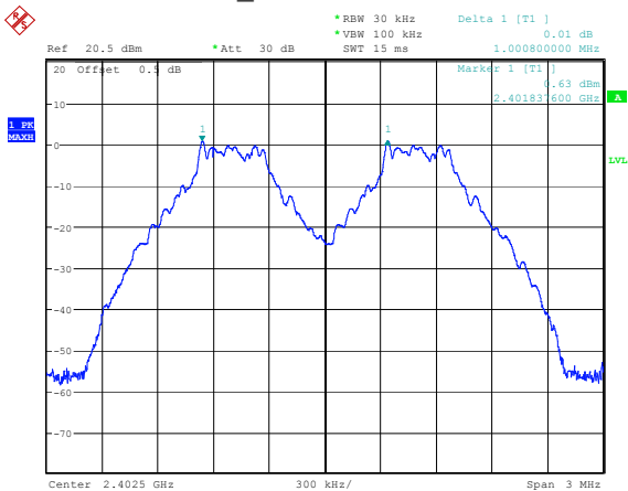
DH1_Low 1.001MHz
