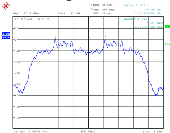
2DH1_Low 1.001MHz
