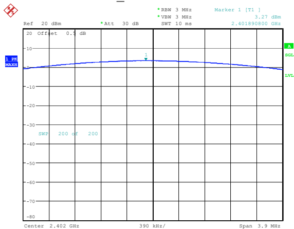
DH1_Low 3.27dBm
