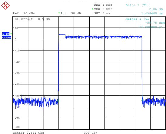
2DH3_Hopping 1.658ms
