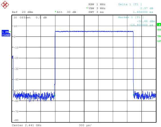
DH3_Hopping 1.656ms
