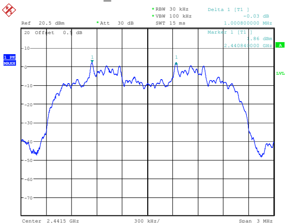
2DH1_Middle 1.001MHz
