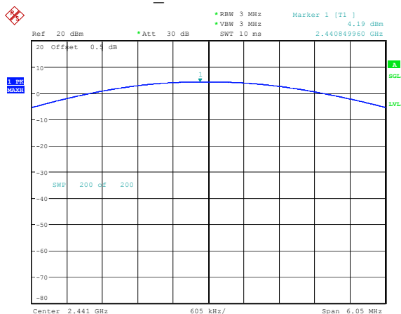
2DH1_Middle 4.19dBm
