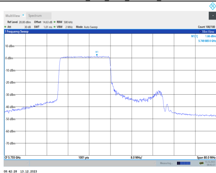
11AX40MIMO Ant2 5755 26Tone RU0
