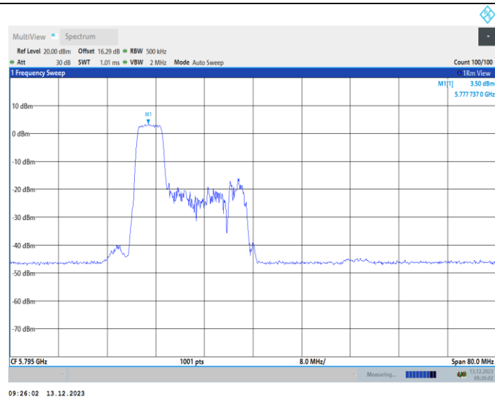
11AX40MIMO Ant2_5795_106Tone_RU53
