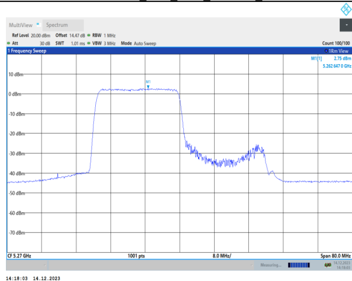
11AX40MIMO Ant2 5270 26Tone RU0
