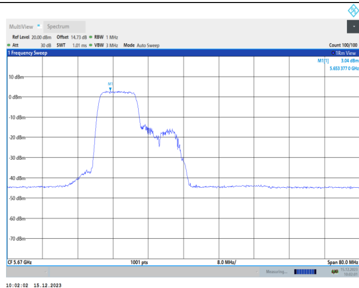
11AX40MIMO Ant2_5670_242Tone_RU61
