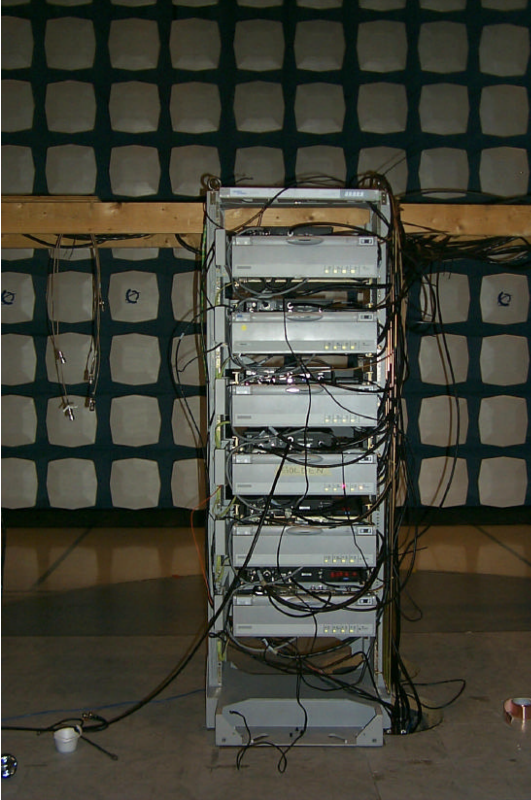
Test Set-up Picture 1: 6 MFRM Radios (Front View)
