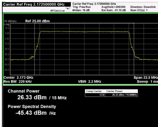
Channel: TOP, Modulation: QPSK, BW=15MHz, Channel Power
