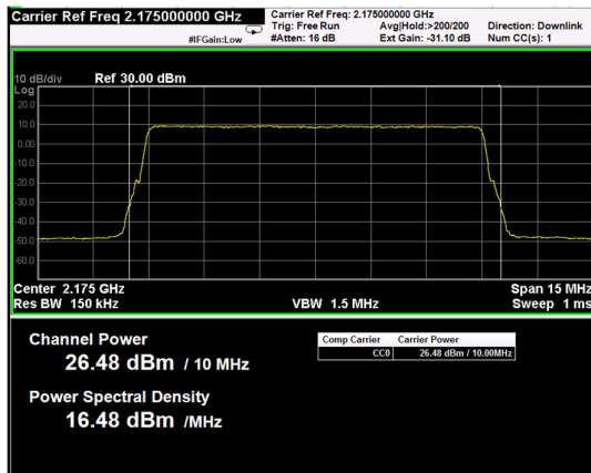
Channel: TOP, Modulation: QPSK, BW=10MHz, Channel Power
