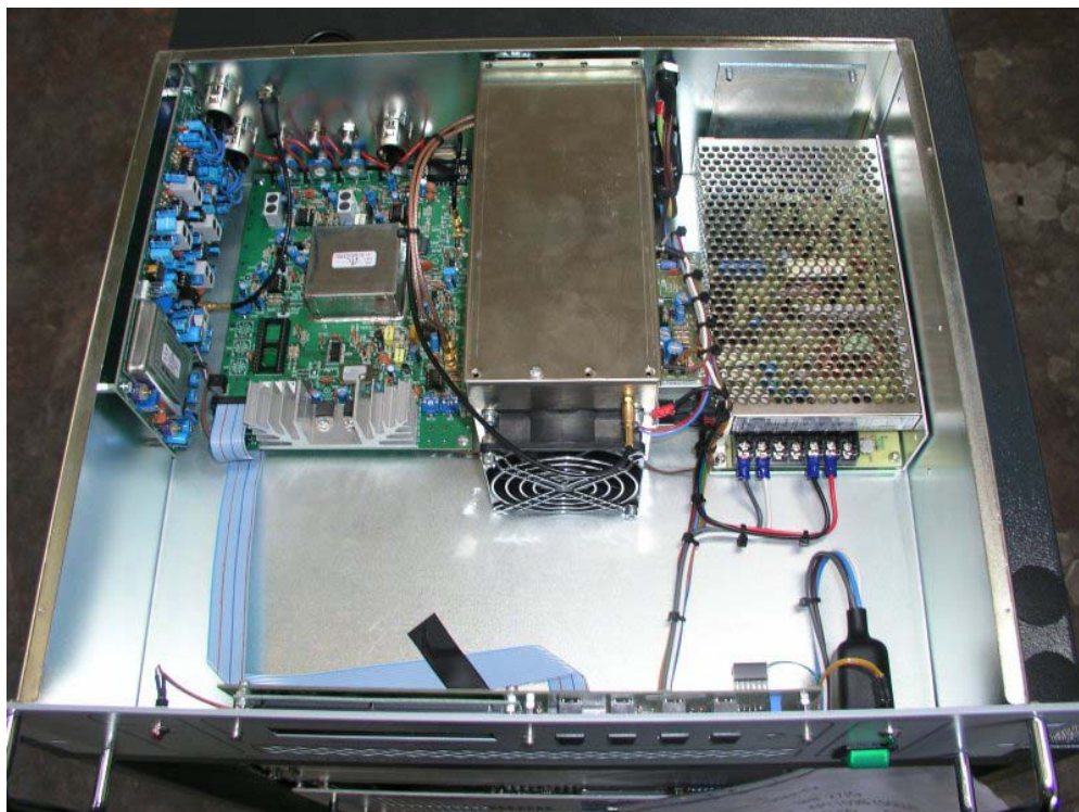
PLLC TOP VIEW
