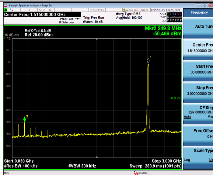
11N20SISO_Ant1_2412_30~3000
