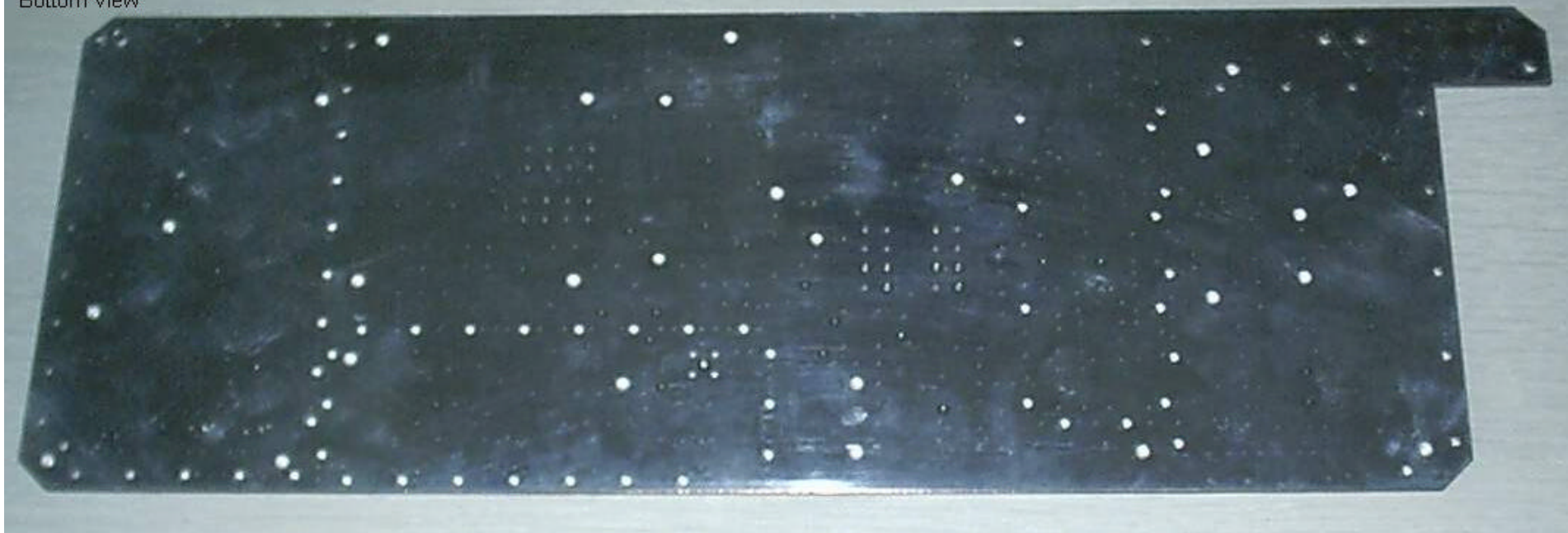
Digivance LRCS 1900 MHz Power Amplifier Loop Board Bottom View
