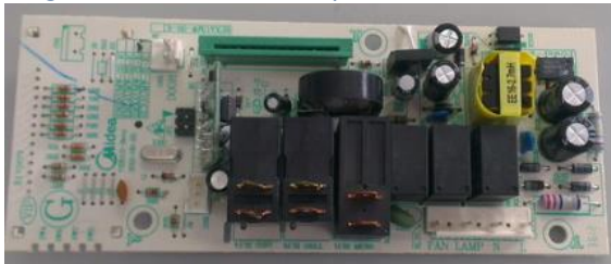
Original Mother board-top view
